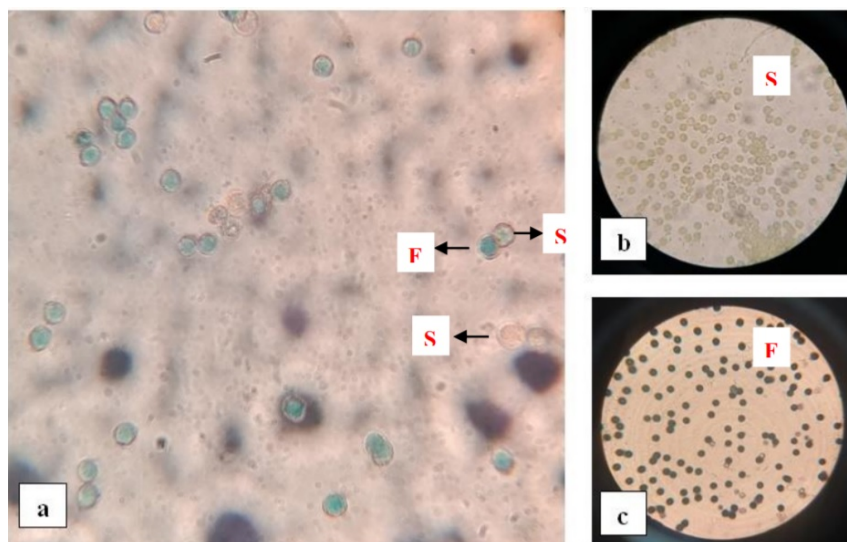
Figure 3. Pollen of gambir type Udang by using bromothymol blue coloring method. (a) Fertile and sterile pollen, (b) sterile pollen, (c) Fertile pollen. Note : F= Fertile, S = Sterile
