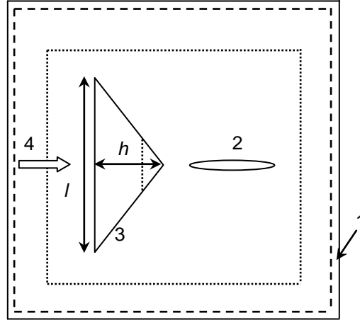
Figure 1: Sketch of the model: 1 – PML; 2 – photonic jet; 3- top view of triangular cylinder; 4 – plane wave. Dot line – border of TF area, while dashed line is border of computational domain.
