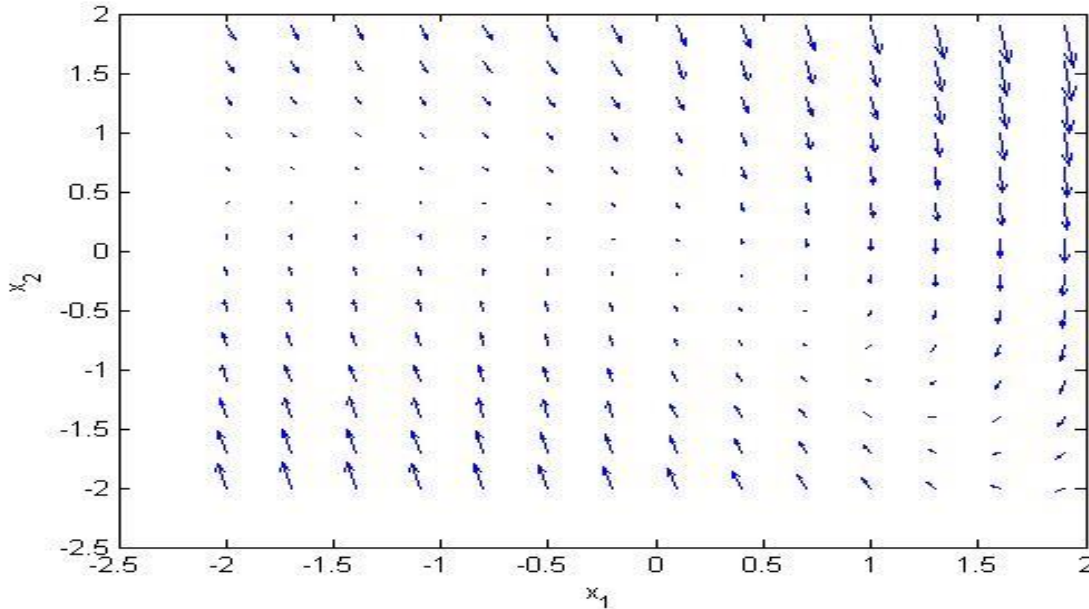
Fig. 2: Phase plane diagram of system 5.3 showing the trajectories of the Eigenvalues
