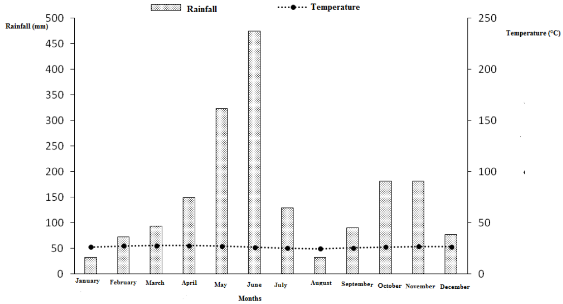
Figure 2. Ombrothermal curve covering the decade from 2006 to 2015 at Station Marc Delorme (SMD)
