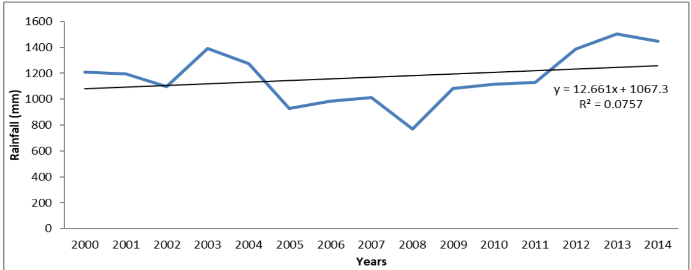
Figure 3: Annual rainfall for Kaduna State (2000 to 2014)
