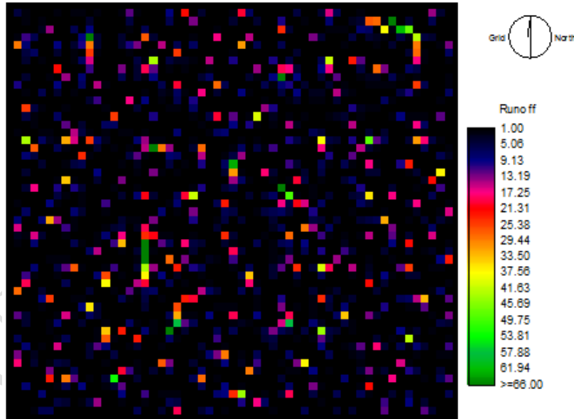
Figure 5: NDVI image showing the amount of runoff (2004)
