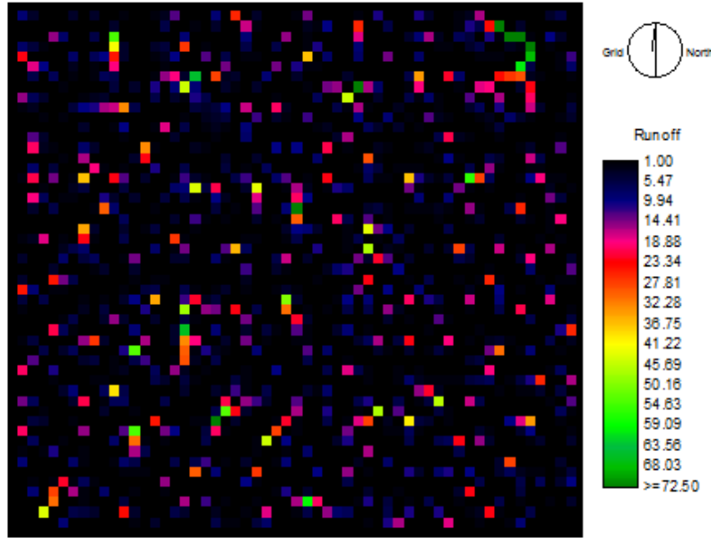
Figure 4: NDVI image showing the amount of runoff (2000)
