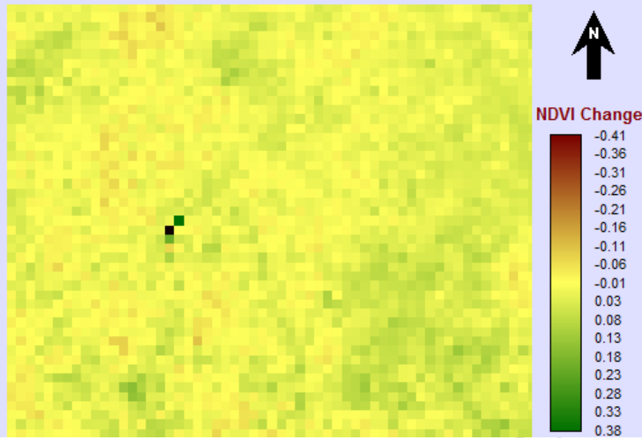
Figure 9: Proportionate long term change image
