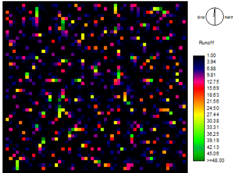
Figure 6: NDVI image showing the amount of runoff (2009)
