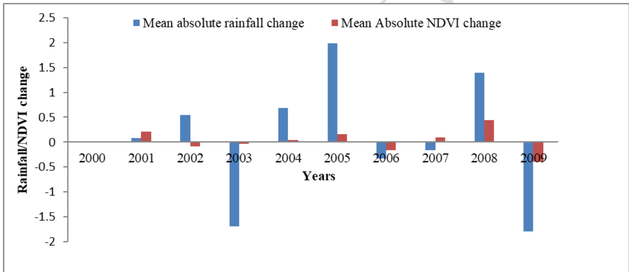
Figure 11: Mean absolute rainfall and NDVI change histogram
