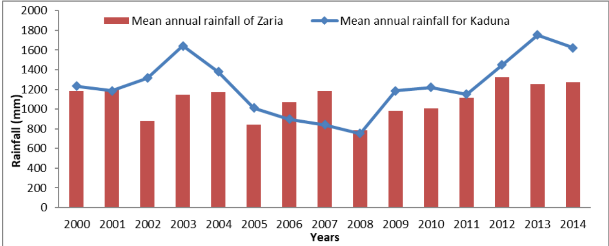
Figure 2: Comparative line and bar graphs showing annual rainfall for Zaria and Kaduna (2000-2014)
