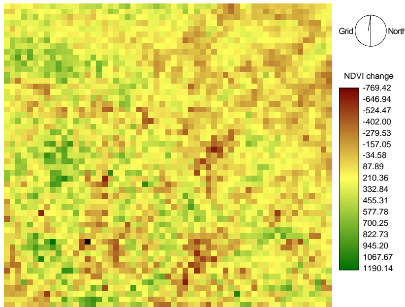
Figure 8: Quasi 5-years change image (2000/2001 to 2004/2005)
