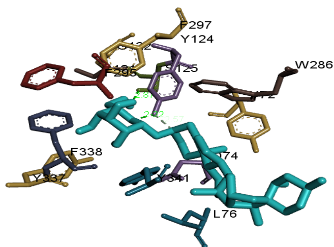
Figure 4: Interaction of Gamma-solamargine docked to the “catalytic site” of the AChE. The ligand (Gsm) has been shown in ‘stick’(sky blue color) representation. Hydrogen bonds shown by green dotted lines.
