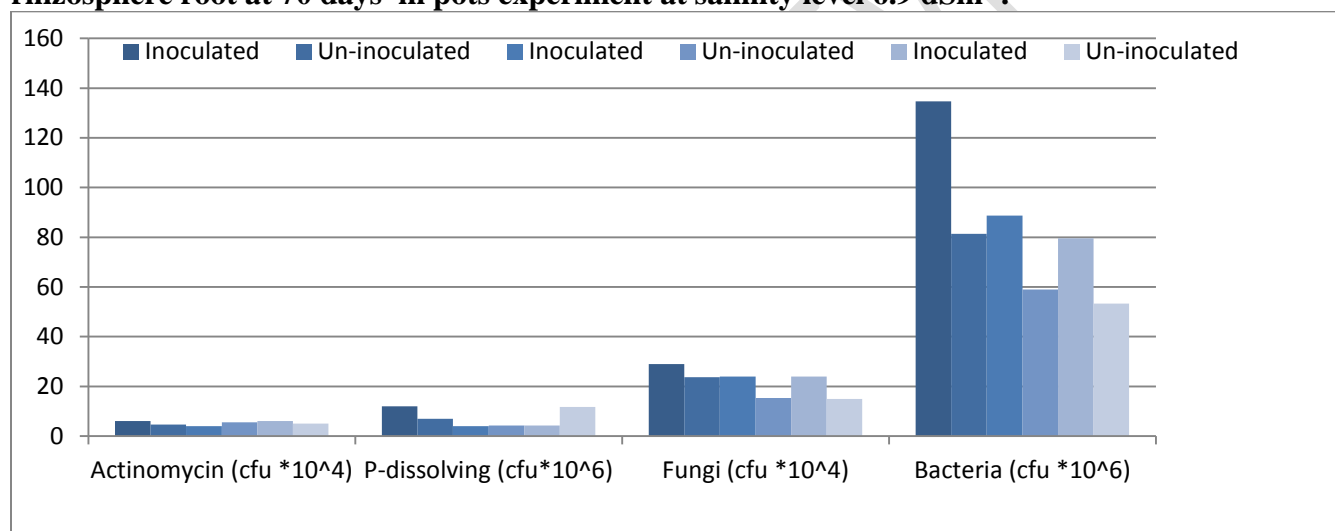
Fig: 3 showed effect of inoculation and phosphorus fertilization on microbial count of faba bean rhizosphere root at 70 days in pots experiment at salinity level 8.7 \text{ dSm}^{-1} .
