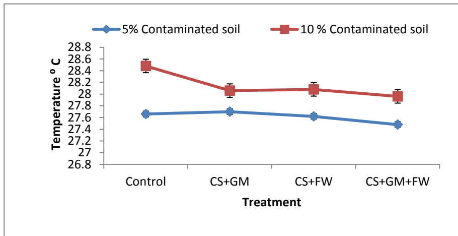
Fig.7: Mean Temperature values for all the set-ups within 56 days
