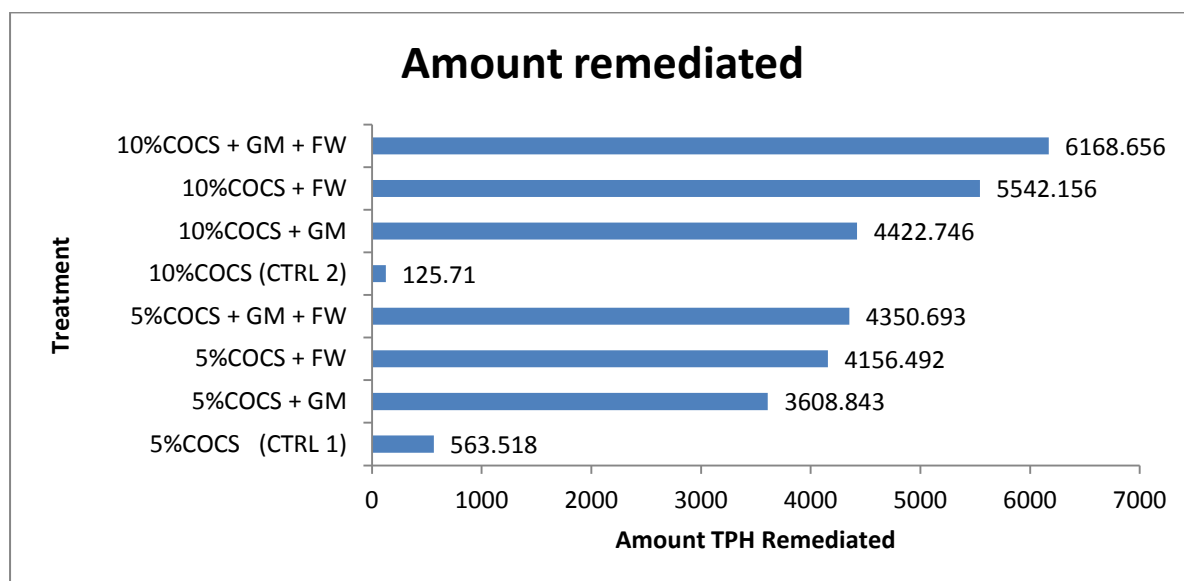
Figure 3: Amount of THP remediation by the Goat Manure and Fish wastein the 5%and 10% Crude oil contaminated soil within 56 days
