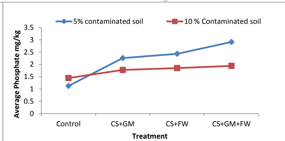
Fig.8: Mean Phosphate values for all the set-ups within 56 days
