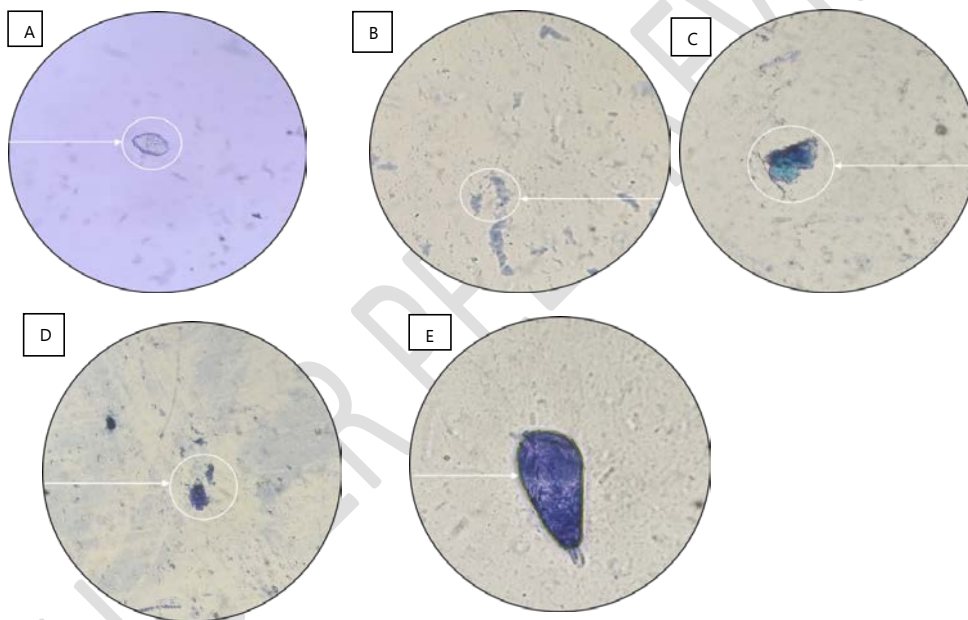
Figure 7: Toxicity Assay performed on Human Cheek Cells (HCCs) shows normal squamous cell (A) in the absence of toxin isolated; deformity in structure was observed in presence of toxin (B-E) [400x magnification].
