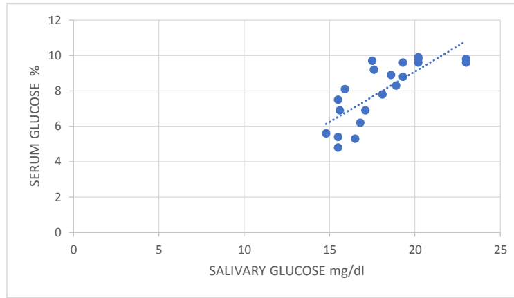
Graph 1: Correlation between salivary and blood glucose levels in the diabetic group
