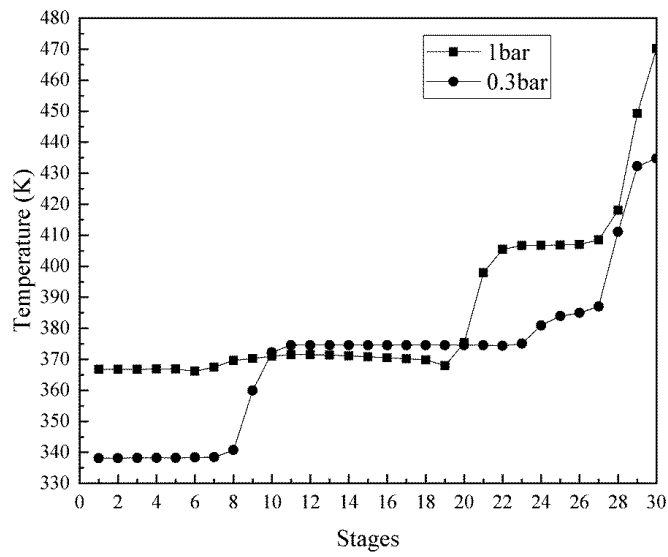
Fig. 3. Temperature profile of the esterification column at 0.3 bar and 1.0 bar ( N_R=7 , N_{rxn}=15 , N_S=8 , Q_R=1700 KW, FR_{iAmOH/Lact}=1:1 )
