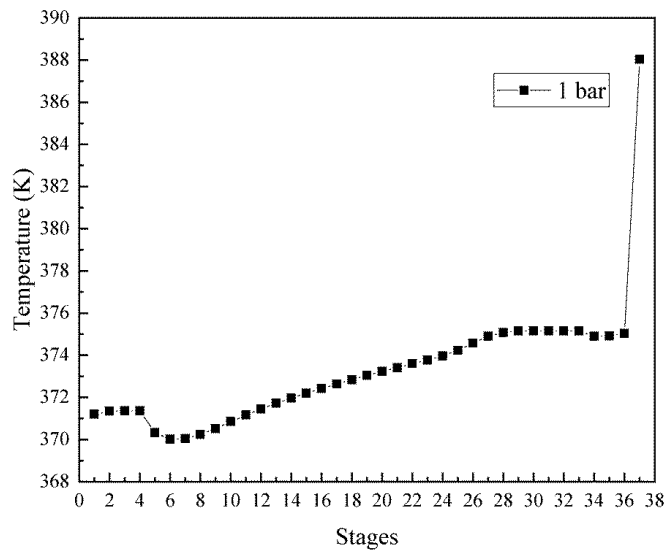
Fig. 4. Temperature profile of the hydrolysis column at 1.0 bar ( N_R=5 , N_{rxn}=40 , N_S=5 , Q_R=1500 KW, FR_{Water/iAmLc}=3:1 )
