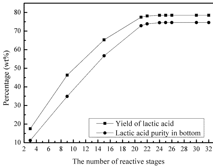
Fig. 6. Effect of reactive stages on the yield and purity of bottom lactic acid in hydrolysis column ( P=1.0 bar, N_R=5 , N_S=5 , Q_R=1500 KW, FR_{Water/iAmLc}=3:1 )
