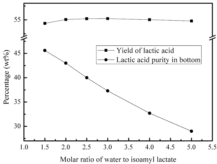
Fig. 9. Effect of FR_{\text{Water/iAmLc}} on the yield and purity of bottom lactic acid in hydrolysis column
