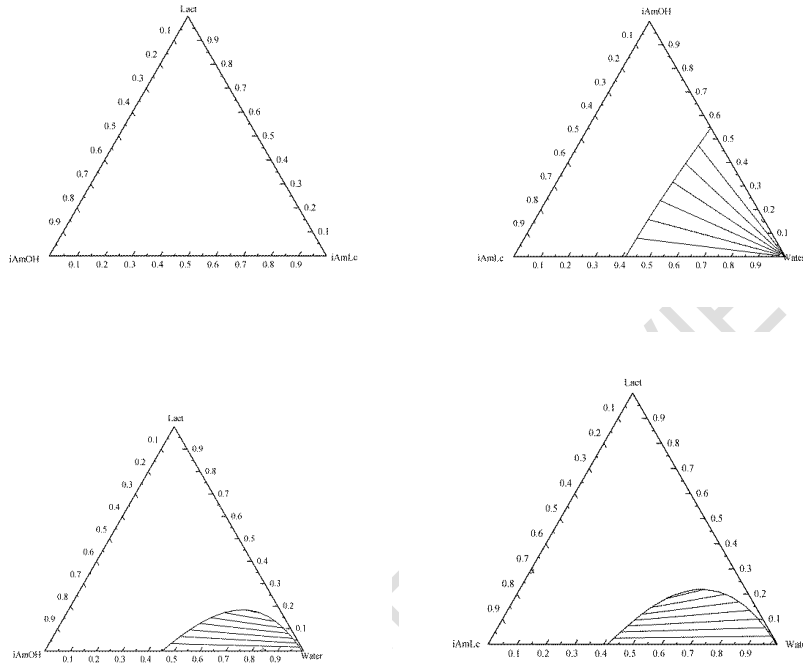
Fig. 1. Ternary diagrams for Lact/iAmOH/water/iAmLc mixture system
