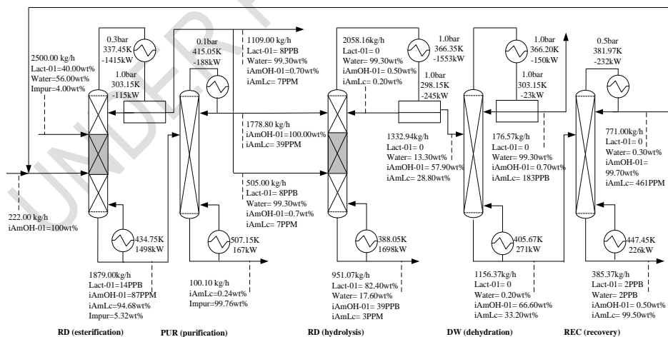
Fig. 12. Simulation results for steady process of the system
