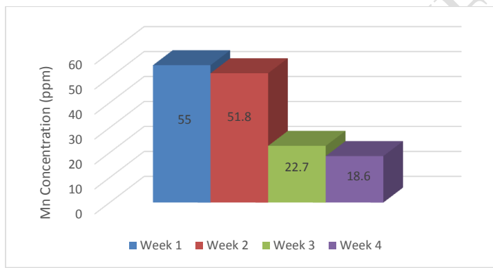
Picture-Figure 1. Weekly concentration of The content of Mn in Lemna Cultivation Media on Every Week
