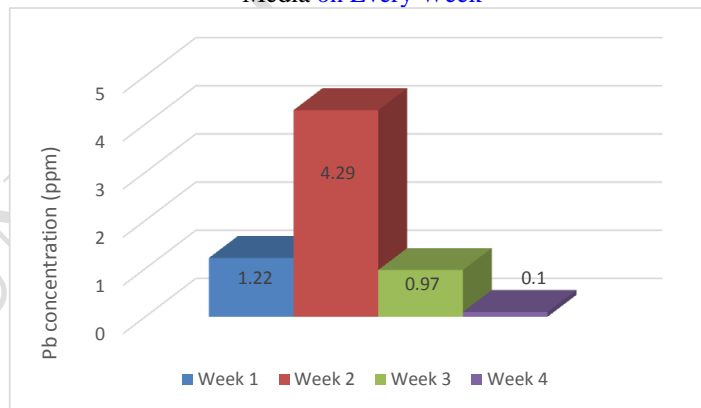
Picture-Figure 2:- Weekly concentration of Pb eontent in Lemna cultivation media every week
