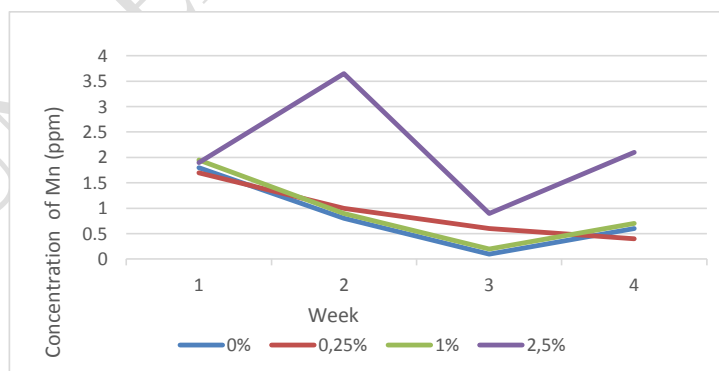
Picture 3. Concentration of Mn Content in Lemna Cultivation Media Shortly After Addition of Bioslurry
