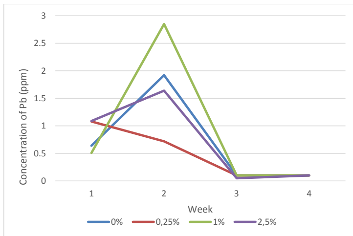
Picture 4. Concentration of Pb Content in Lemna Cultivation Media Shortly After Addition of Bioslurry
