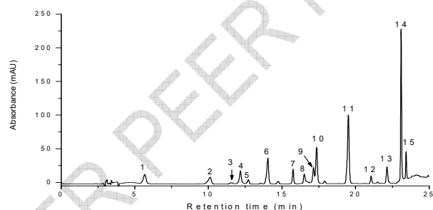
Fig. 1. Chromatogram of standards (0.1mg/mL)
