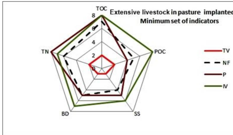
193 TOC: total organic carbon; POC: particulate organic carbon; SS: structural stability; BD: 194 bulk density; TN: total nitrogen; TV: threshold values; NF: native forest; P: pasture; IV: 195 initial values. 196
