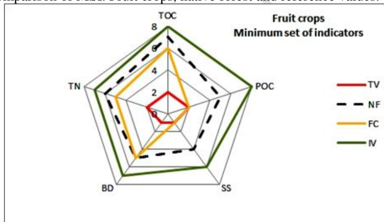
199 TOC: total organic carbon; POC: particulate organic carbon; SS: structural stability; BD: 200 bulk density; TN: total nitrogen; TV: threshold values; NF: native forest; FC: fruit crops; IV: 201 initial values. 202
