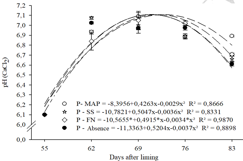
Figure. 1: PH values (CaCl) in the different sources of phosphate fertilization (MAP, SS, and FN) as a function of incubation time.
