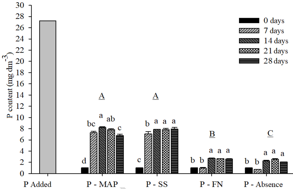
Figure. 2: For the phosphorus contents, there was a significant difference between the fertilization sources and the evaluation time.
