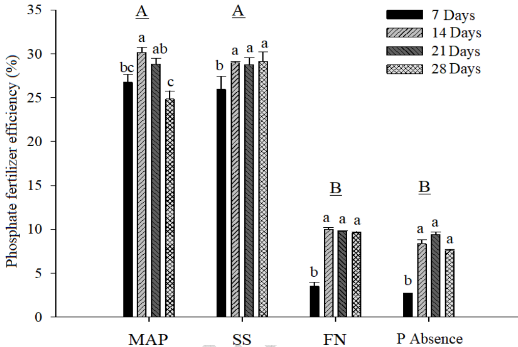
Figure. 3: The efficiency of different sources of phosphate fertilizers as a function of sources and epochs.
