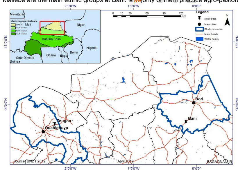
Fig. 1. Phytogeographic map and situation of the experimental site in Northern Burkina Faso
