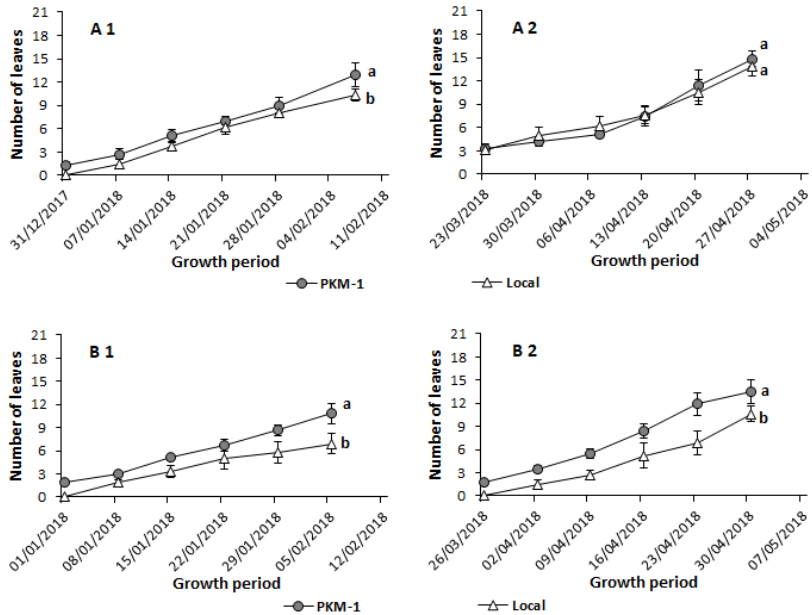
Fig. 2. Weekly average increase in mean number of leaves per plant of the different varieties of Moringa (PKM1 and Local) during the first month of the trials at Bani (A1, A2) and Tougou (B1, B2).
