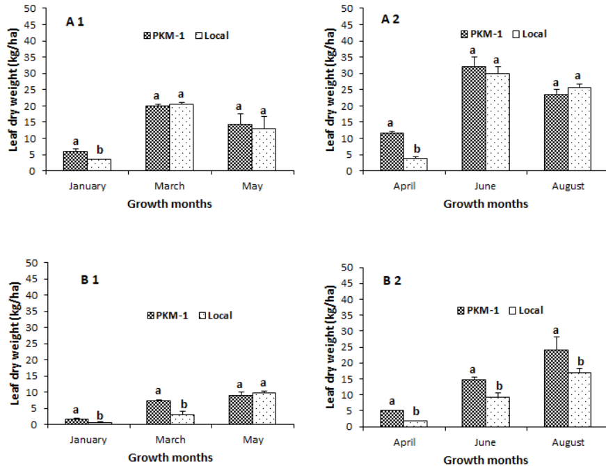
Fig. 4. Leaf dry biomass production of the different varieties of Moringa (PKM-1 and Local) at the sites of Bani (A1, A2) and Tougou (B1, B2).
