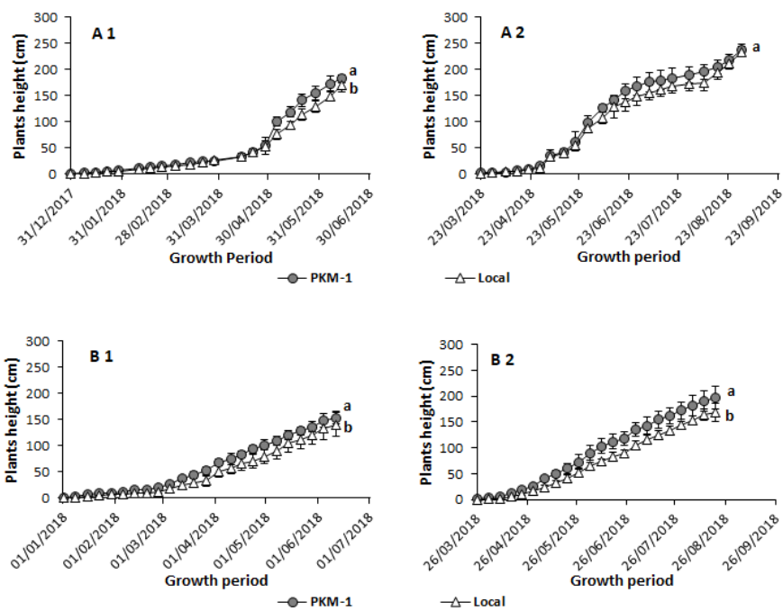
Fig. 3. Monthly average increase in mean seedlings' heights (cm) of the different varieties of Moringa (PKM-1 and Local) at the sites of Bani (A1, A2) and Tougou (B1, B2).
