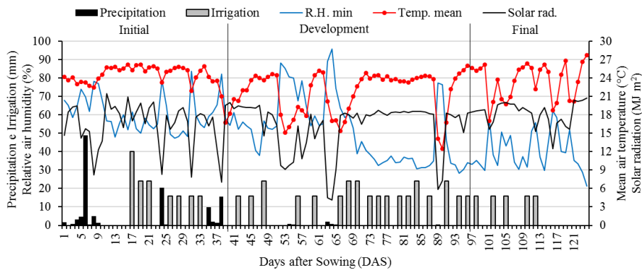
Fig. 1. Mean air temperature, Precipitation, Irrigation, Solar radiation and Relative air humidity, during the experimental period in Tangará da Serra—MT, 2018
