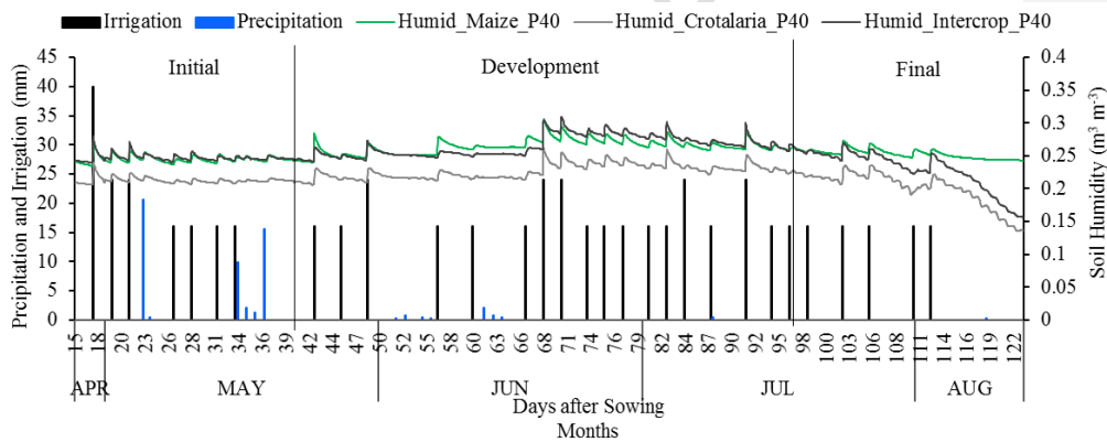
Fig. 5. Soil moisture variability at a depth of 0.40 m and accumulated rainfall and irrigation during the crop cycle
