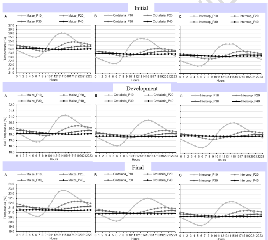
Fig. 3. Hourly variation of the soil temperature at depths 0.10, 0.20, 0.30 and 0.40 m, in (A) maize, (B) Crotalaria-C. juncea and (C) intercropping systems, in relation to phenological stages of culture, initial, development and final
