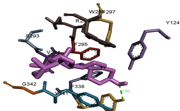
Figure 3: Interaction of solanidine docked to the “catalytic site” of the AChE. The ligand has been shown in ‘stick’(purple color) representation. The hydrogen bond is shown by green dotted lines.
