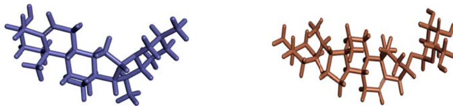
Figure 2: Chemical structure of Solanidine and Gamma-solamargine
