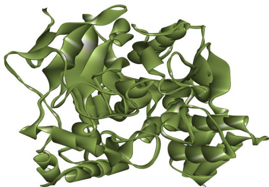
Figure 1: The 3-D structure of recombinant human acetylcholinesterase enzyme
