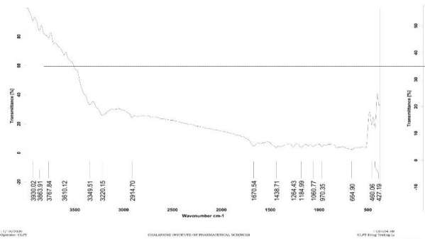
Fig. 1. FTIR of Pure Drug Favipiravir
