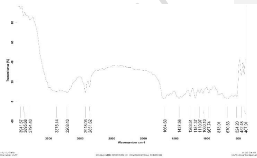
FIG 4 FTIR of Pure drug and MCC
