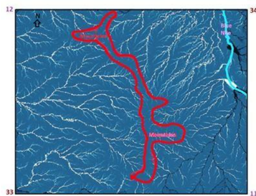
Fig. 5, The drainage network in the study area.
