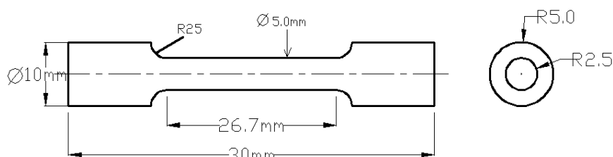
Figure 1 Tensile Strength Test specimen
