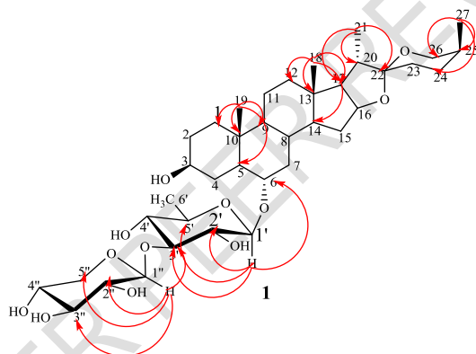
Figure 2. HMBC correlations of compound 1
