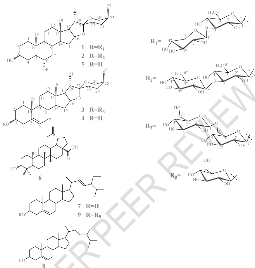
Figure 1. Chemical structures of isolated compounds 1–9
