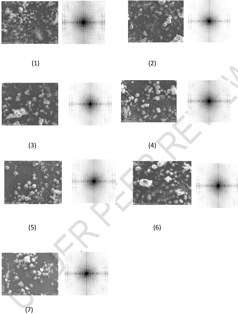
Figure 5: SEM photographs and the Fourier Transform of seven millets: 1-Barnyard, 2-Browntop, 3-Foxtail, 4-Kodo, 5-Little, 6-Pearl, 7-Proso.
