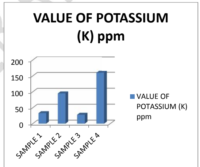
Fig.8 – Value of available Potassium (K) in soil samples
