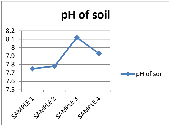
Fig.5-pH of soil samples.
