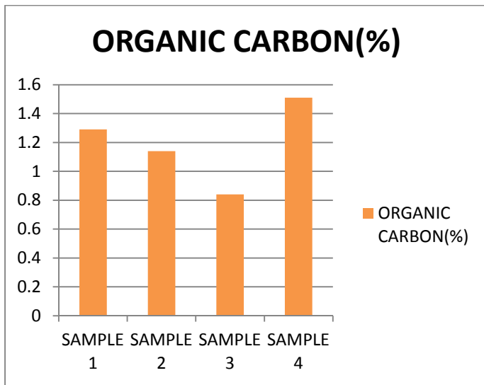
Fig. 7 - Organic carbon % in soil samples.
