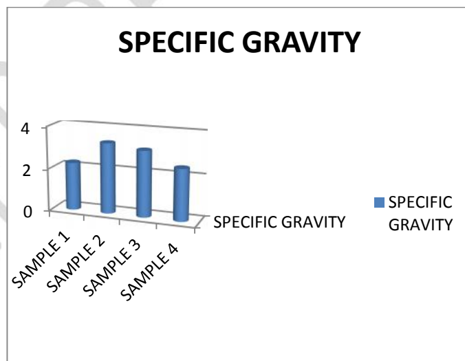
Fig.4. Specific gravity (unitless) of soil sample.
