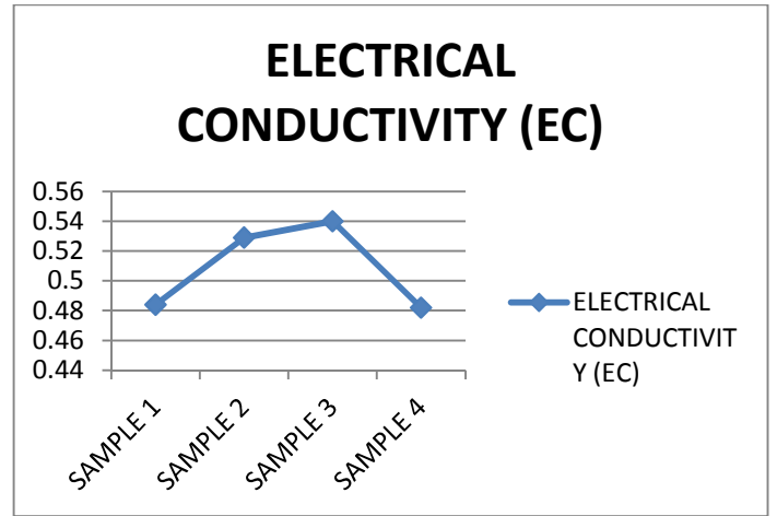
Fig.6- Electrical conductivity ( \text{d Sm}^{-1} ) of soil samples.
