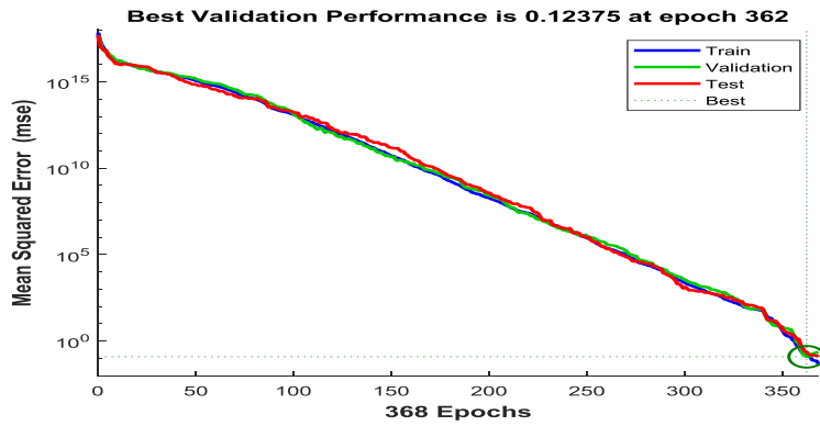
Fig 5: Plot performance for the Hybrid model
