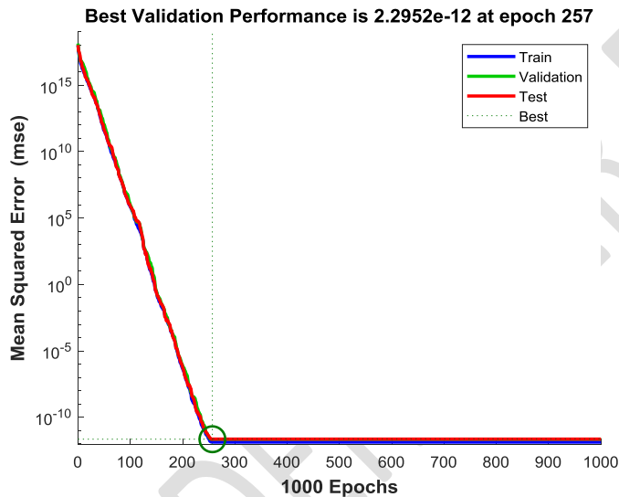
Fig 3: Plot performance for network architecture 6:3:1
