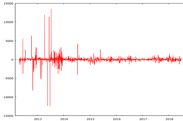
Fig. 1: Time plot of differenced data
