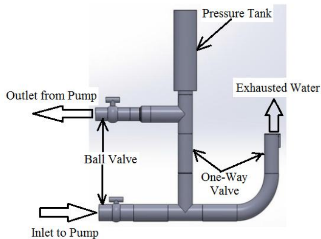
Fig. 1 Schematic of the hydraulic ram pump
