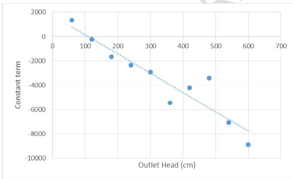
Fig. 7. Variation of constant term coefficient with pump outlet head
