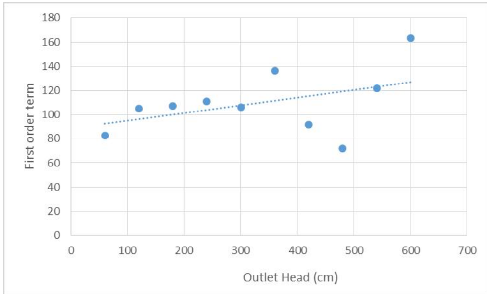
Fig. 6. Variation of first order coefficient with pump outlet head
