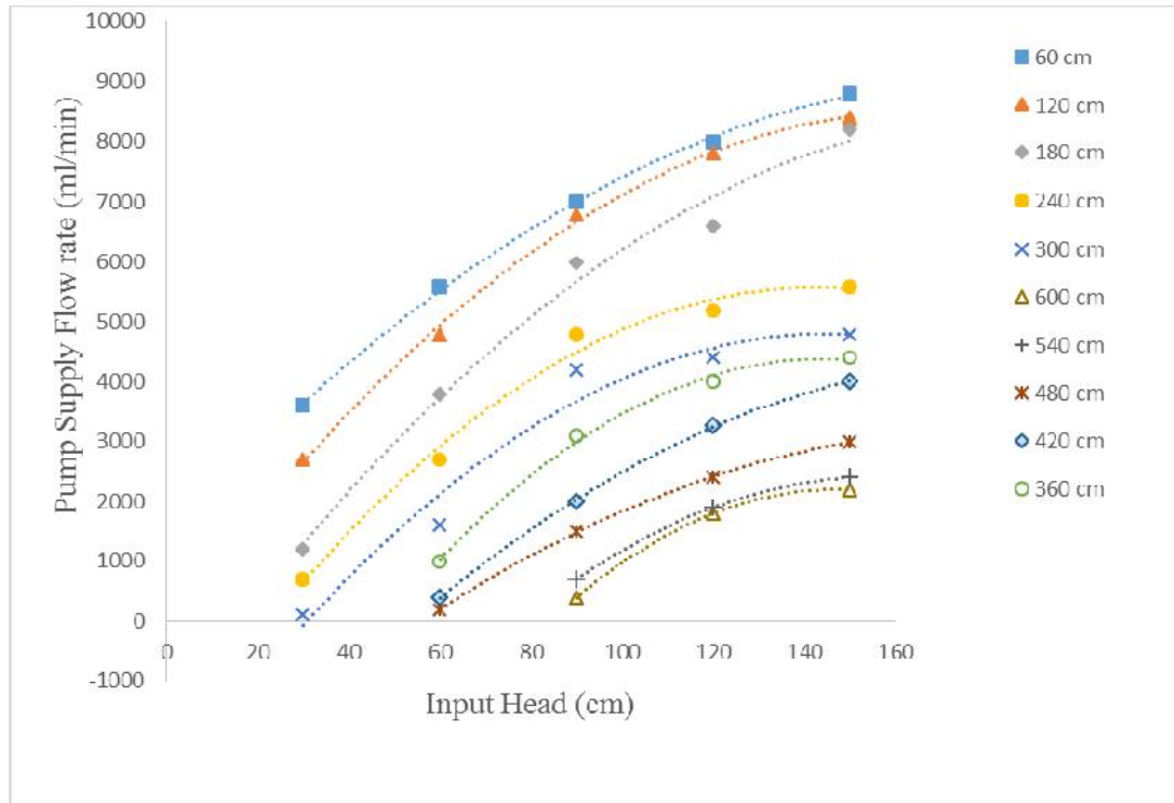
Fig. 4. Plot and least squares best fit line for pump supply flow rate vs. input head
