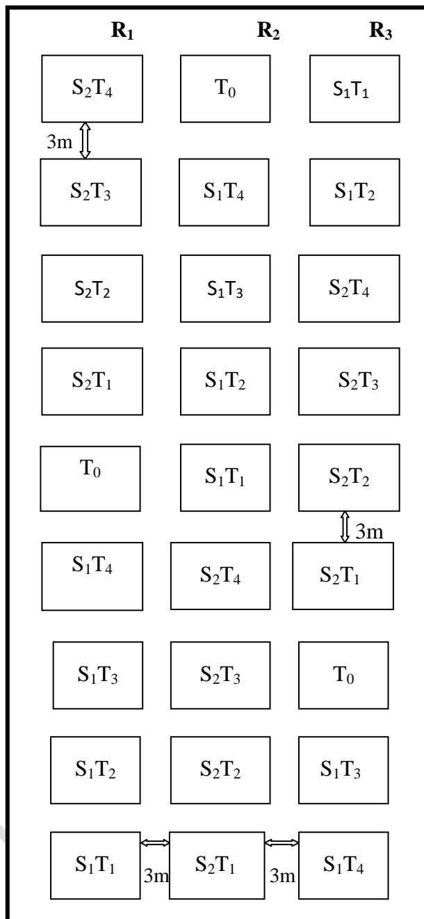
Fig. 1: Layout of the experimental plot
