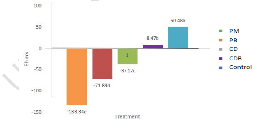
Fig. 4: Average Eh values in terrace soil as influenced by different organic materials during 14 weeks of incubation
