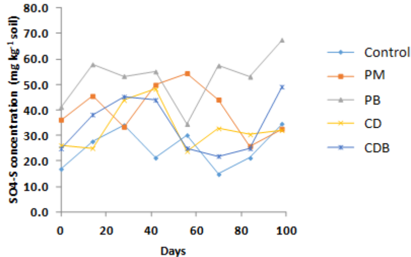
Fig. 7. SO 4 -2 S release in terrace soil as influenced by different organic materials during 14 weeks of incubation
