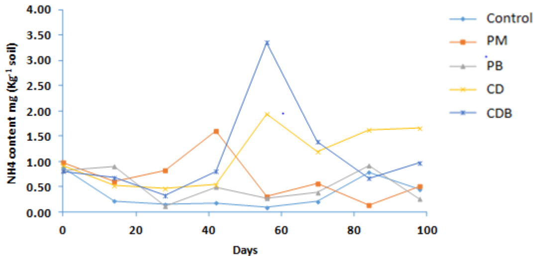
Fig. 5. NH 4 -N release in terrace soil as influenced by different organic materials during 14 weeks of incubation
