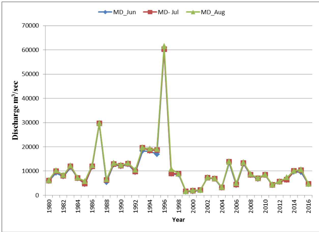
Figure 8. Time series plots for monthly maximum stream flow (summer season) at Sangam Gauging station.
