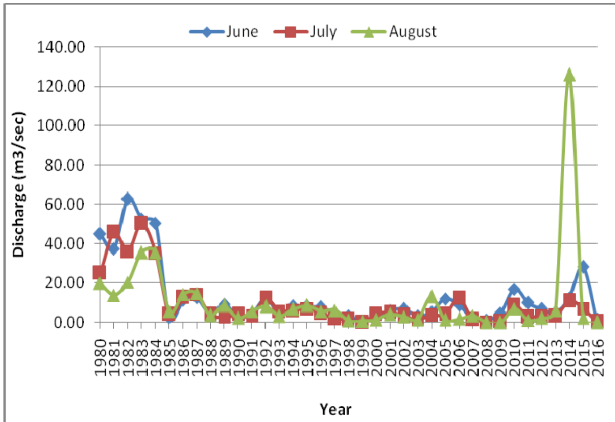
Figure 9. Time series plots for monthly maximum stream flow (summer season) at Verinag Gauging station.
