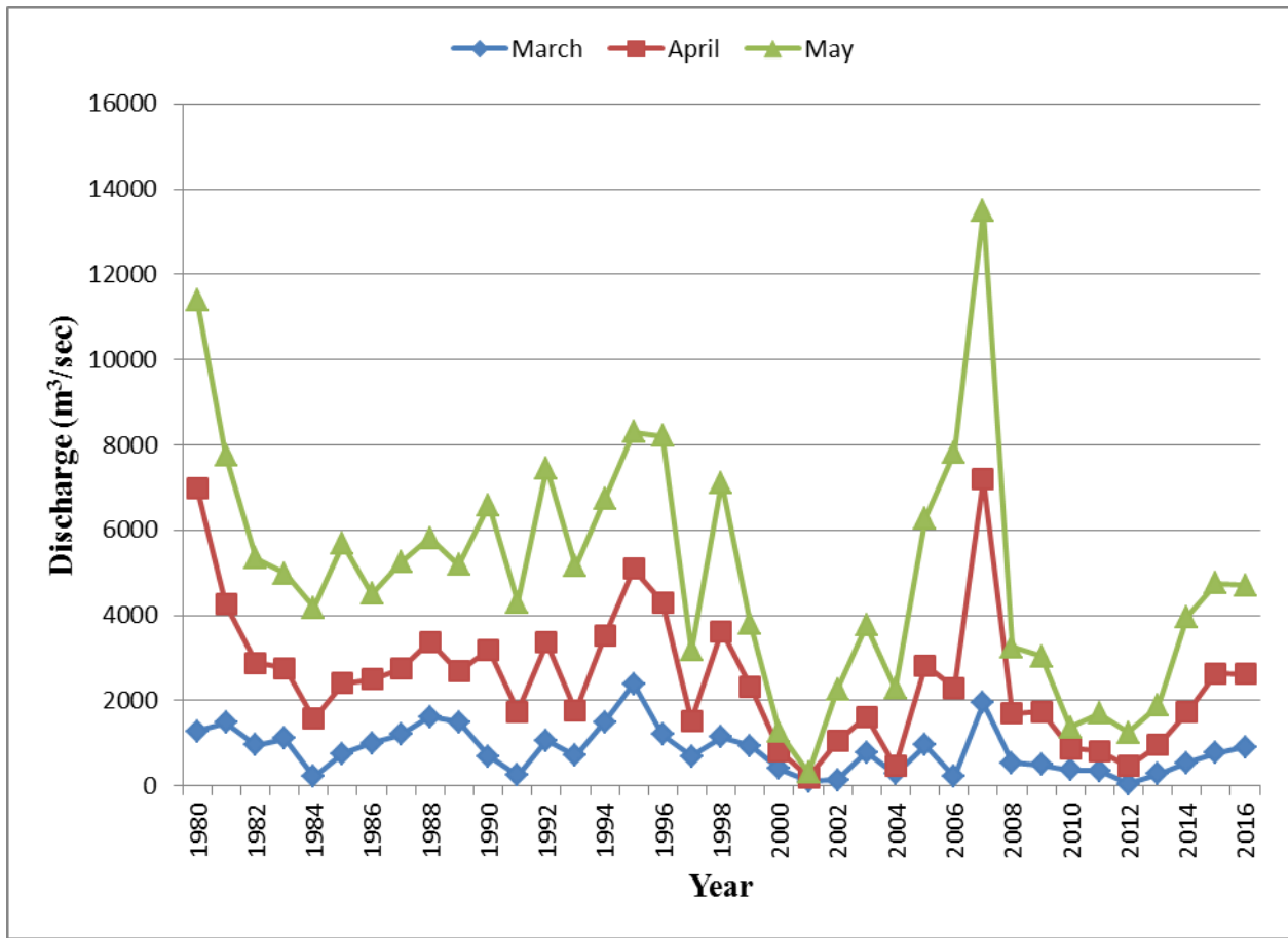
Figure 5. Time series plot for monthly maximum stream flow at Batkoot Gauging station.
