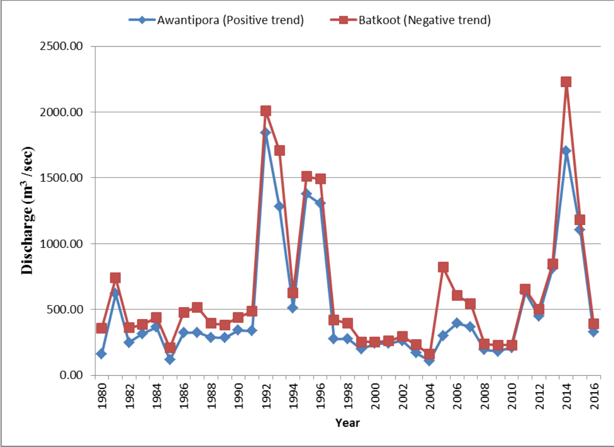
Figure 4. Time series plot for annual maximum stream flow at Awantipora and Batkoot Gauging stations.
