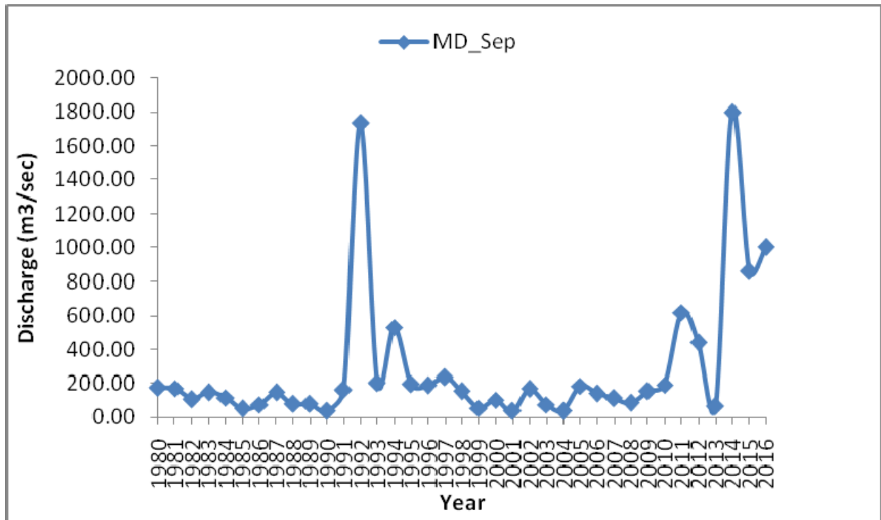
Figure 10. Time series plots for monthly maximum stream flow (autumn season) at Pampore Gauging station.
