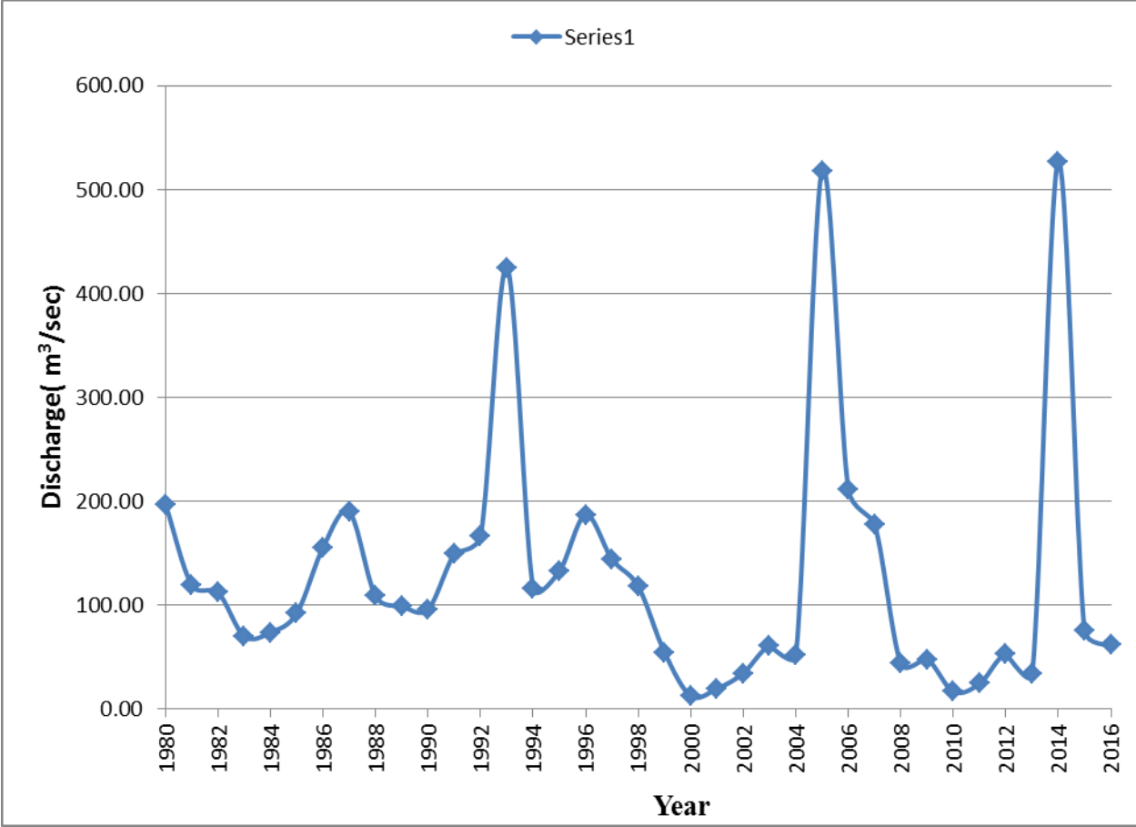
Figure 3. Time series plot for annual maximum stream flow at Arwani Gauging station.
