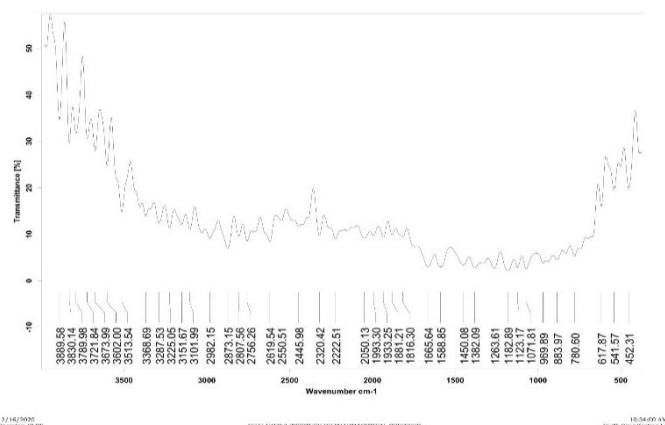
Fig. 2. FTIR spectra of mixture favipiravir and HPMC E50
