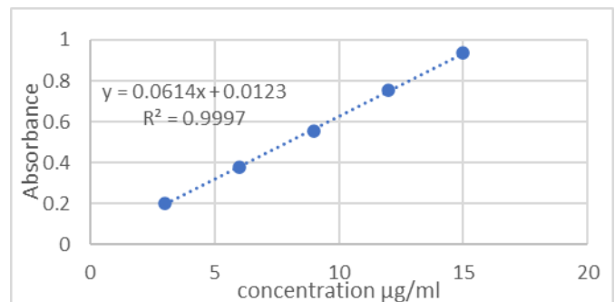
Graph. 1. Standard calibration graph of favipiravir
