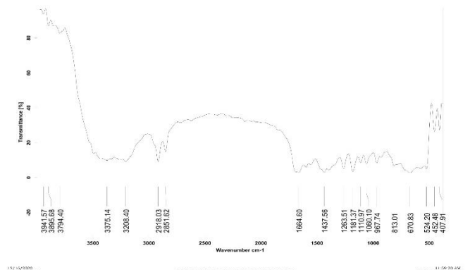
Fig. 4. FTIR spectra of mixture favipiravir and MCC
