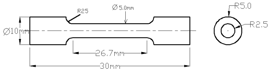
Fig. 1. Tensile Strength Test specimen
