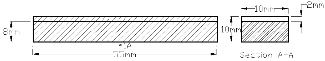
Fig. 2. Impact test specimens of dimensions
