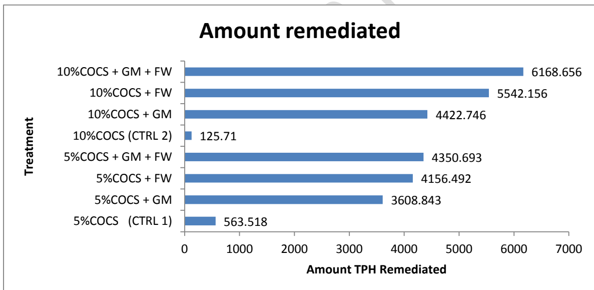
Figure 3: Amount of TPH remediation by the Goat Manure and Fish waste in the 5%and 10% Crude oil contaminated soil within 56 days
