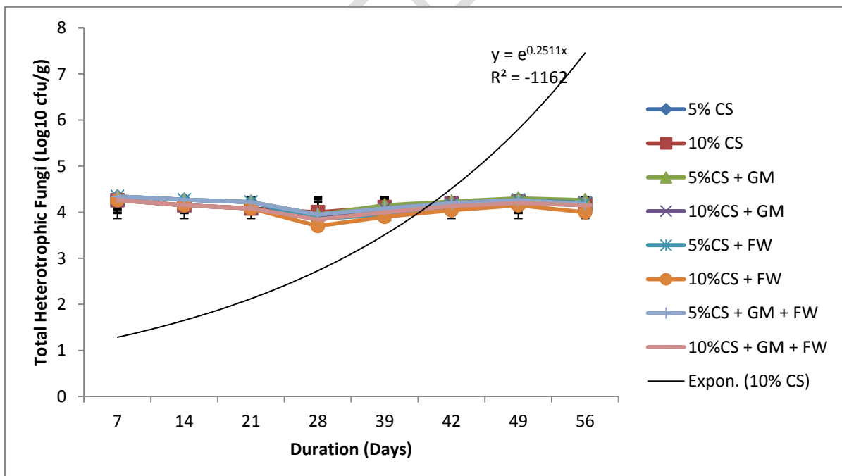
Figure 12: Changes in Total Heterotrophic Fungi ( \log_{10} cfu/g) count during the 56 days of monitoring of the contaminated soil.
