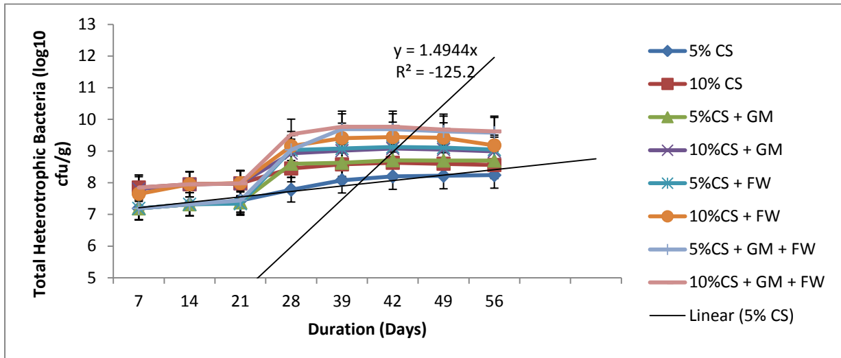
Figure 11: Total Heterotrophic Bacteria ( \log_{10} cfu/g) count during the 56 days of monitoring of the contaminated soil
