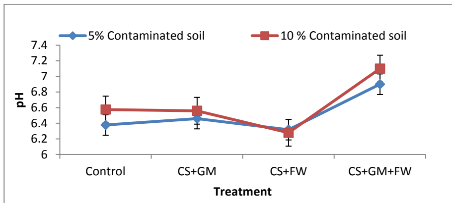
Fig.5: Mean pH values for all the set-ups within 56 days
