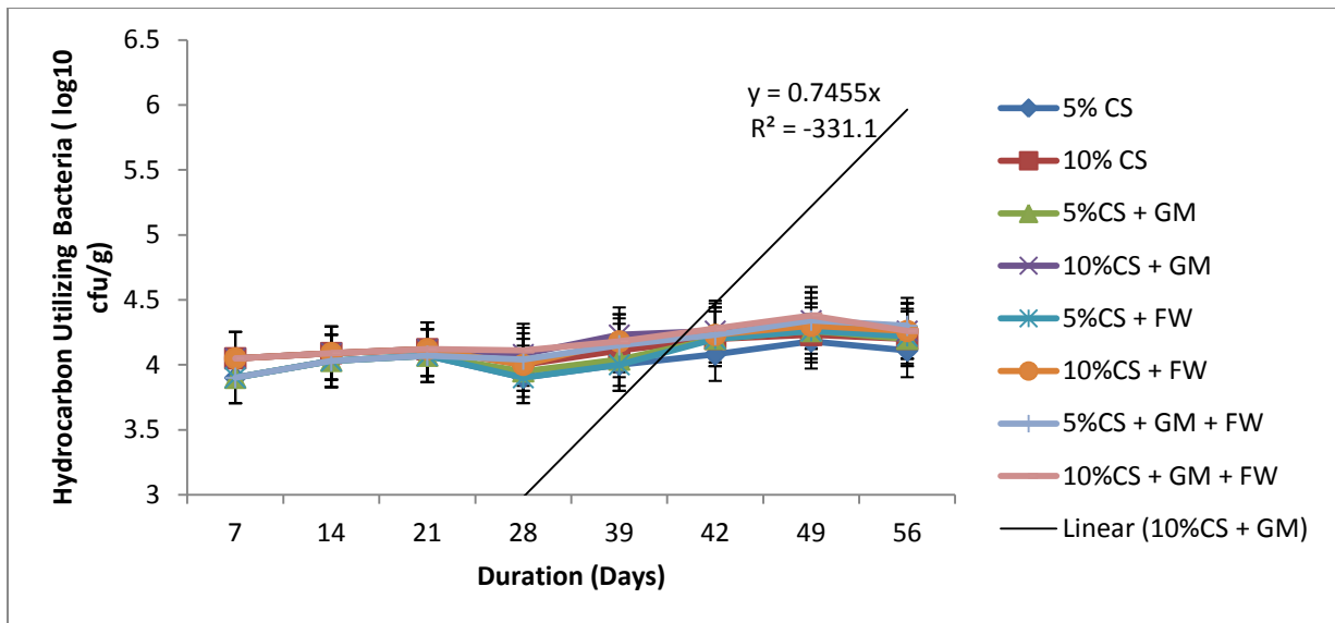
Figure 13: Changes in the Hydrocarbon Utilizing Bacteria ( \log_{10} cfu/g) count during the 56 days of monitoring of the contaminated soil
