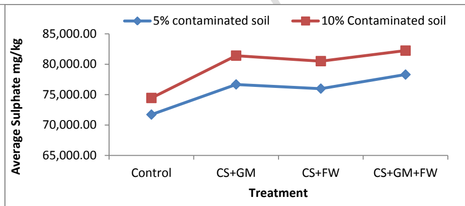
Fig.6: Mean sulphate values for all the set-ups within 56 days
