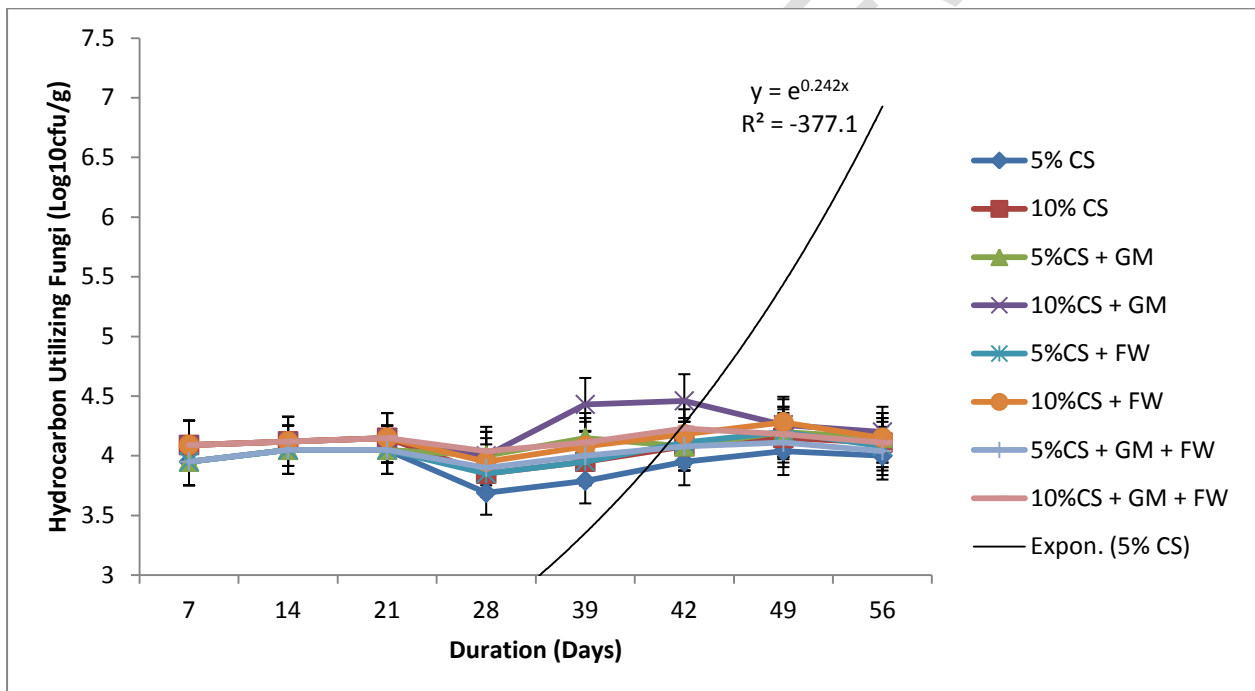
Figure 14: Changes in the Hydrocarbon Utilizing Fungi ( \log_{10} cfu/g) count during the 56 days of monitoring of the contaminated soil
