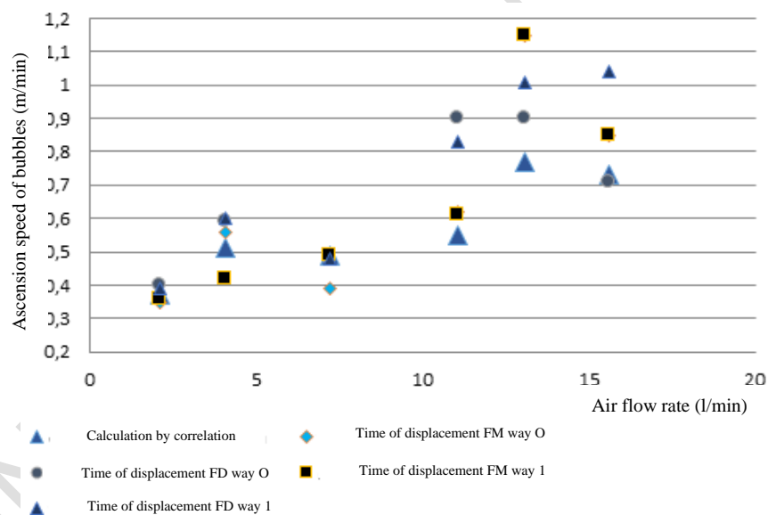
Figure 2: Bubble speed as a function of different calculation mode
