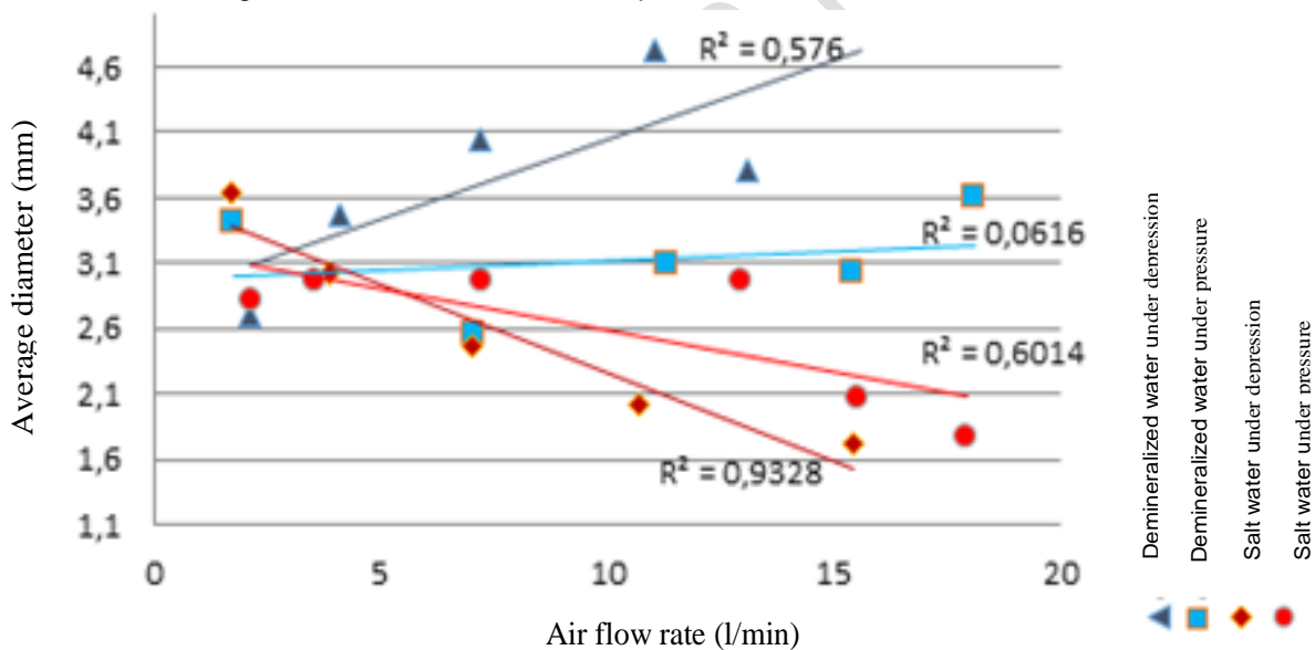
Figure 6: Particle size study for different flow rates
