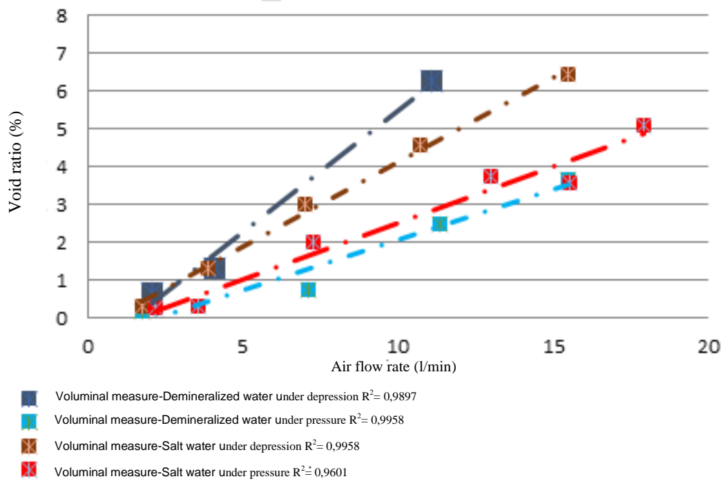
Figure 10: Evolution of the empty rate depending on the type of water
