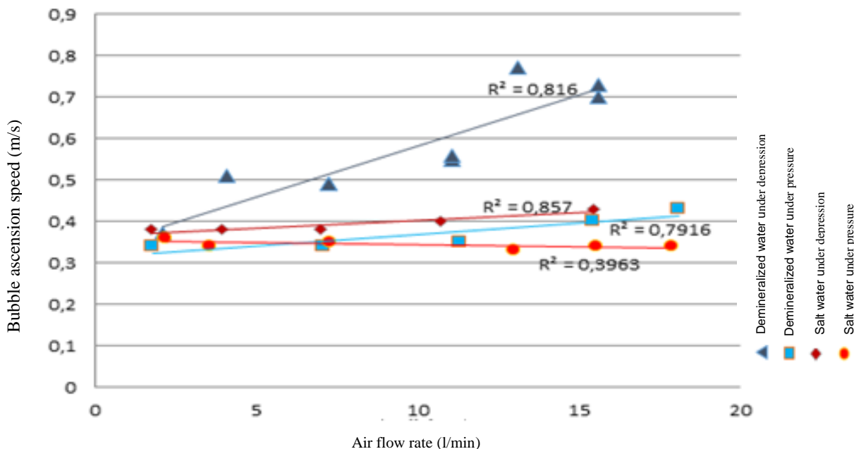
Figure 7: Bubble velocity for different air flow rates
