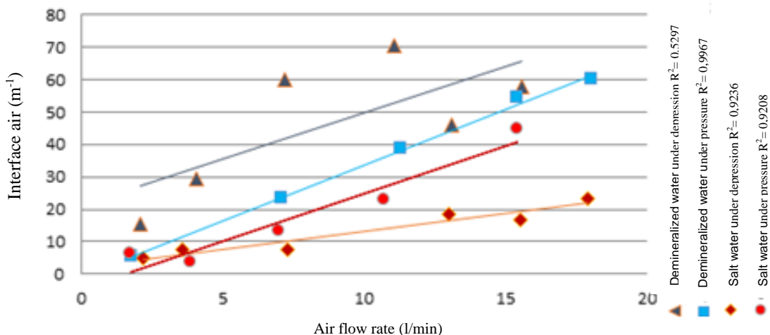
Figure 8: Variation of interfacial air as a function of air flow
