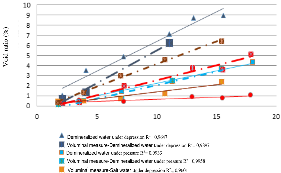
Figure 11: Calculation of the vacuum rate as a function of the air flow
