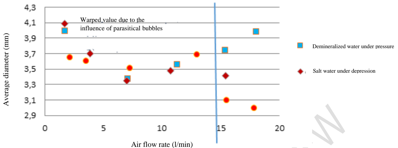
Figure 5: Bubble diameters for different types of water
