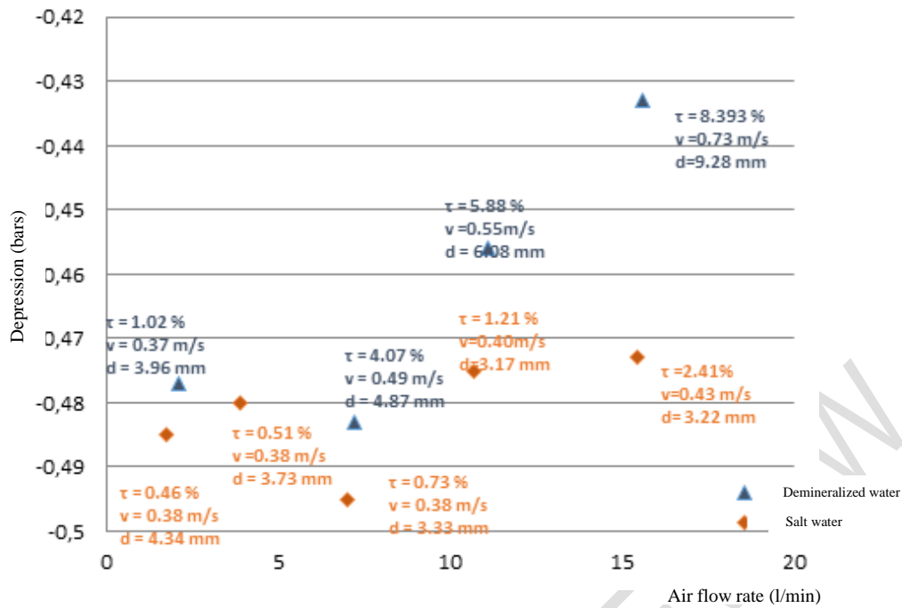
Figure 3: Pressure variation as a function of flow
