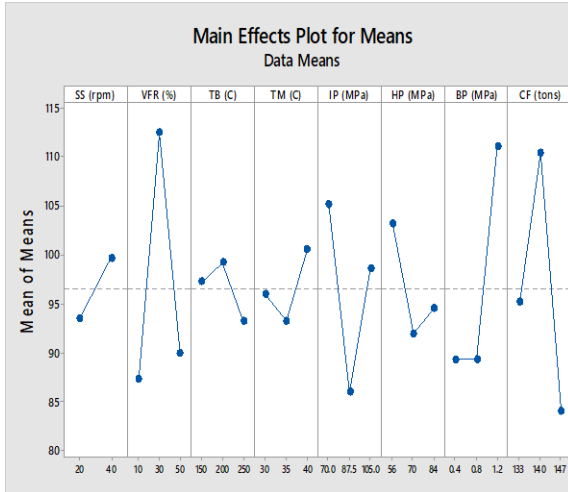
Fig. 1: Main Effects Plot of Signal-to-Noise (Larger is Better) for Flexural Response Particle Size 1
