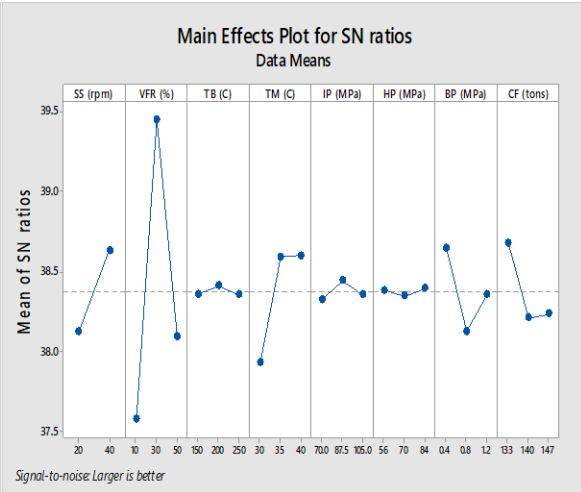
Fig. 2: Main Effects Plot of Means for Flexural Response Particle Size 1
