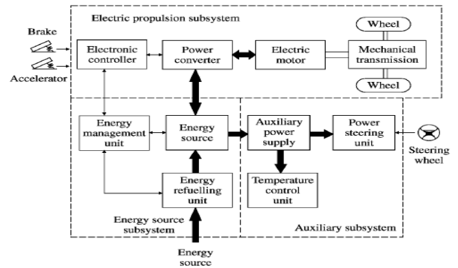
Figure 1 Block diagram of electric vehicle
