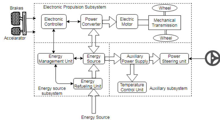
Figure 1 Block diagram of an electric vehicle [13]
