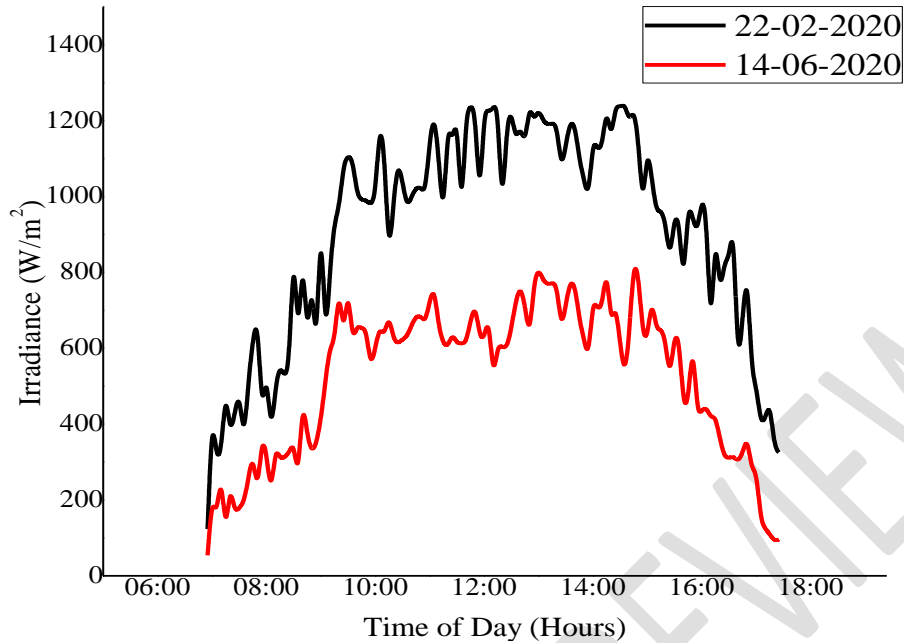
Figure 3: Typical daily solar irradiance at the site.
