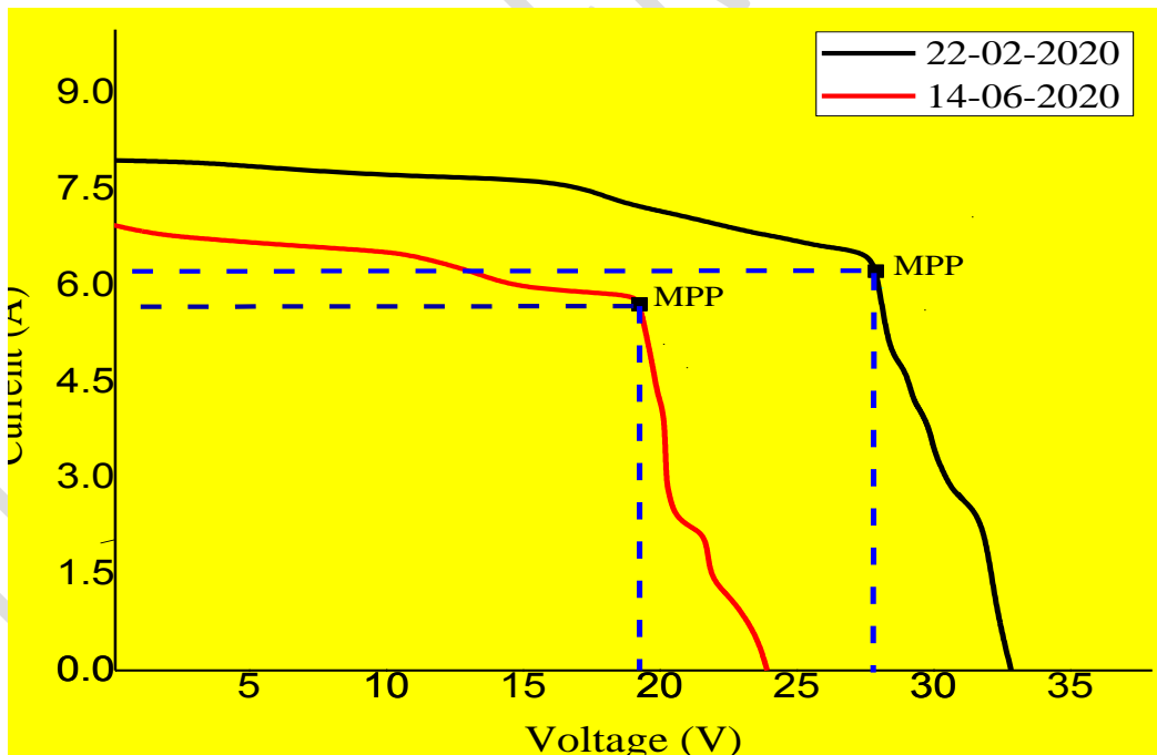
Figure 4: Typical I - V characteristic of the PV backup system.
