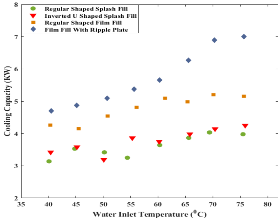
Figure 12. Cooling Capacity vs Water InletTemperature
