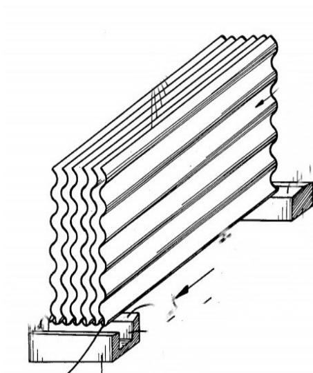
Figure 2. Regular shaped filmfill[11]
