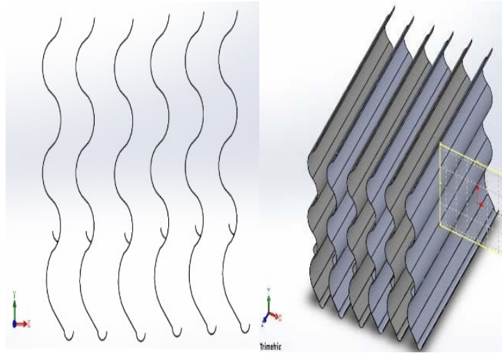
Figure 4. Modified shape film fill with ripple plates
