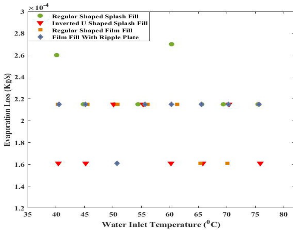
Figure 13. Evaporation Loss vs Water InletTemperature
