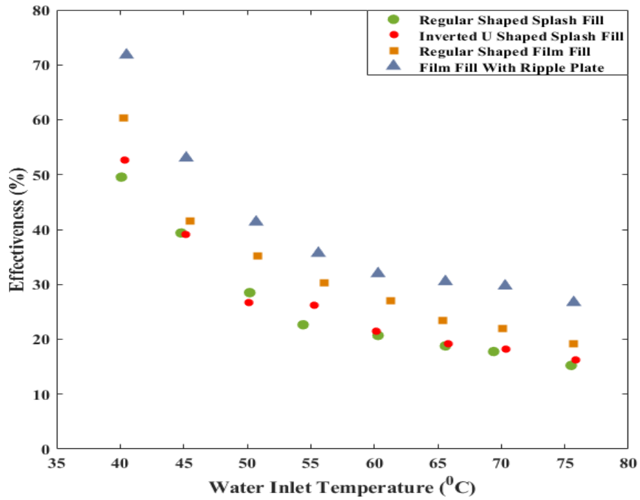
Figure 11. Effectiveness vs Water Inlet Temperature
