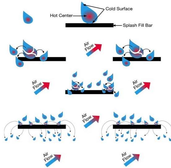
Figure1. Regular shaped splash fill [12]
