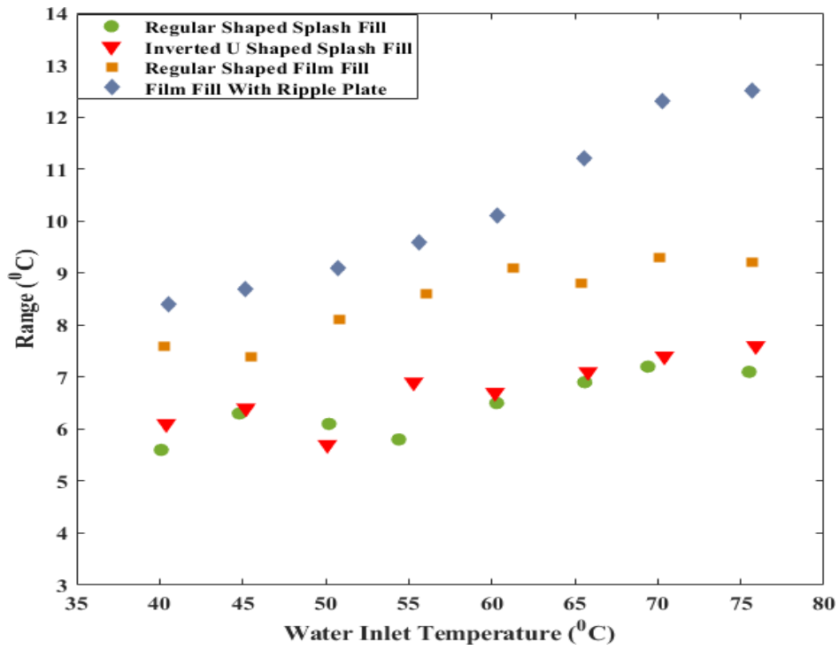
Figure 10. Range vs Water Inlet Temperature
