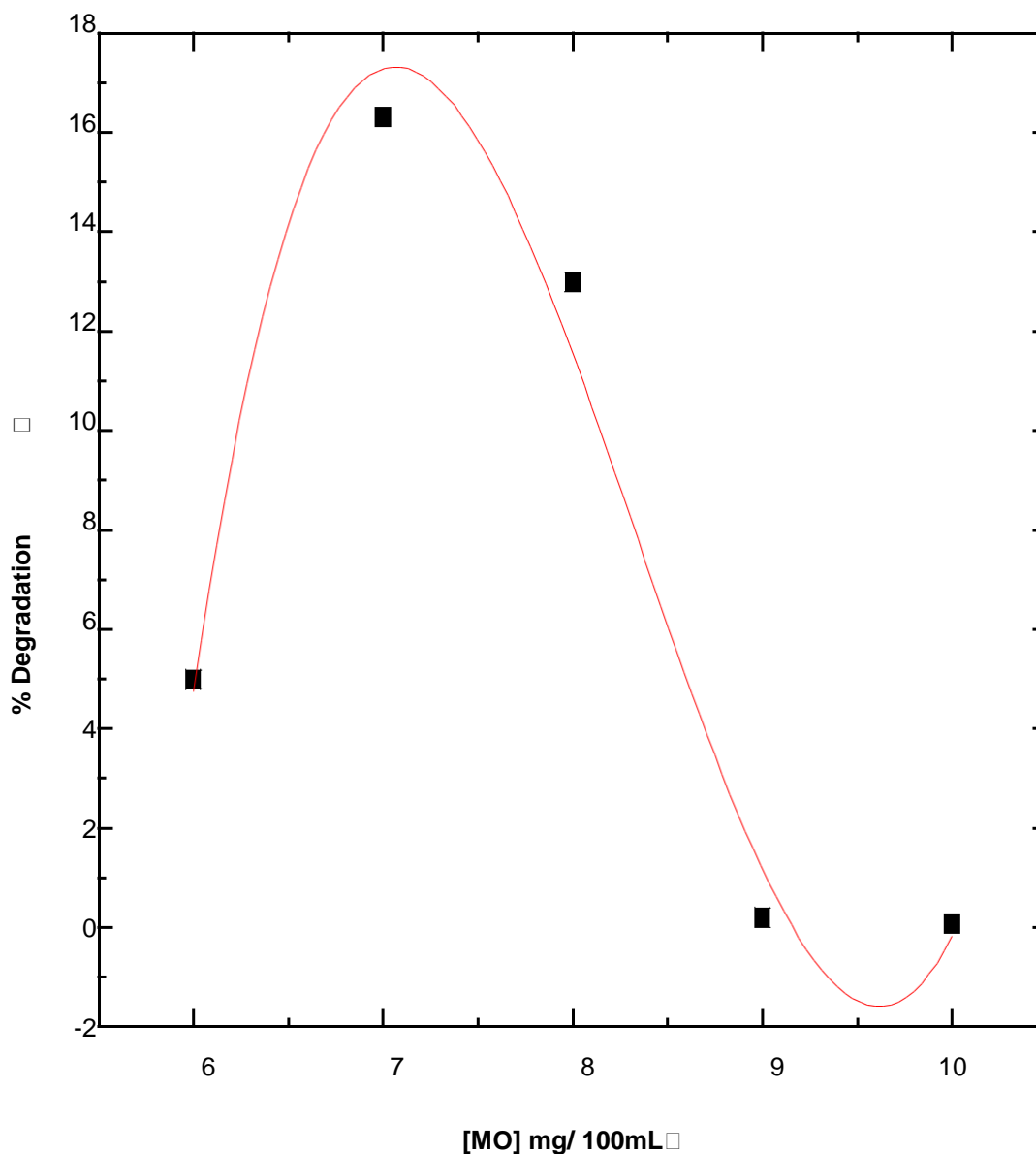
Fig: 3.3(a) Effect of initial concentration of MO on % percentage of degradation during 60 minutes of irradiation
