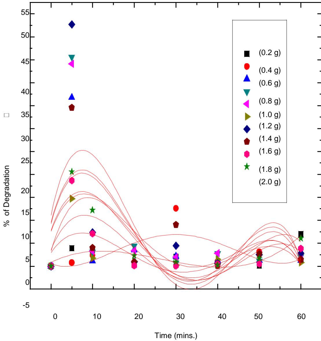
Fig. 3.1(a) the percentage of degradation of the solution with time using at different amount of ZnO suspension
