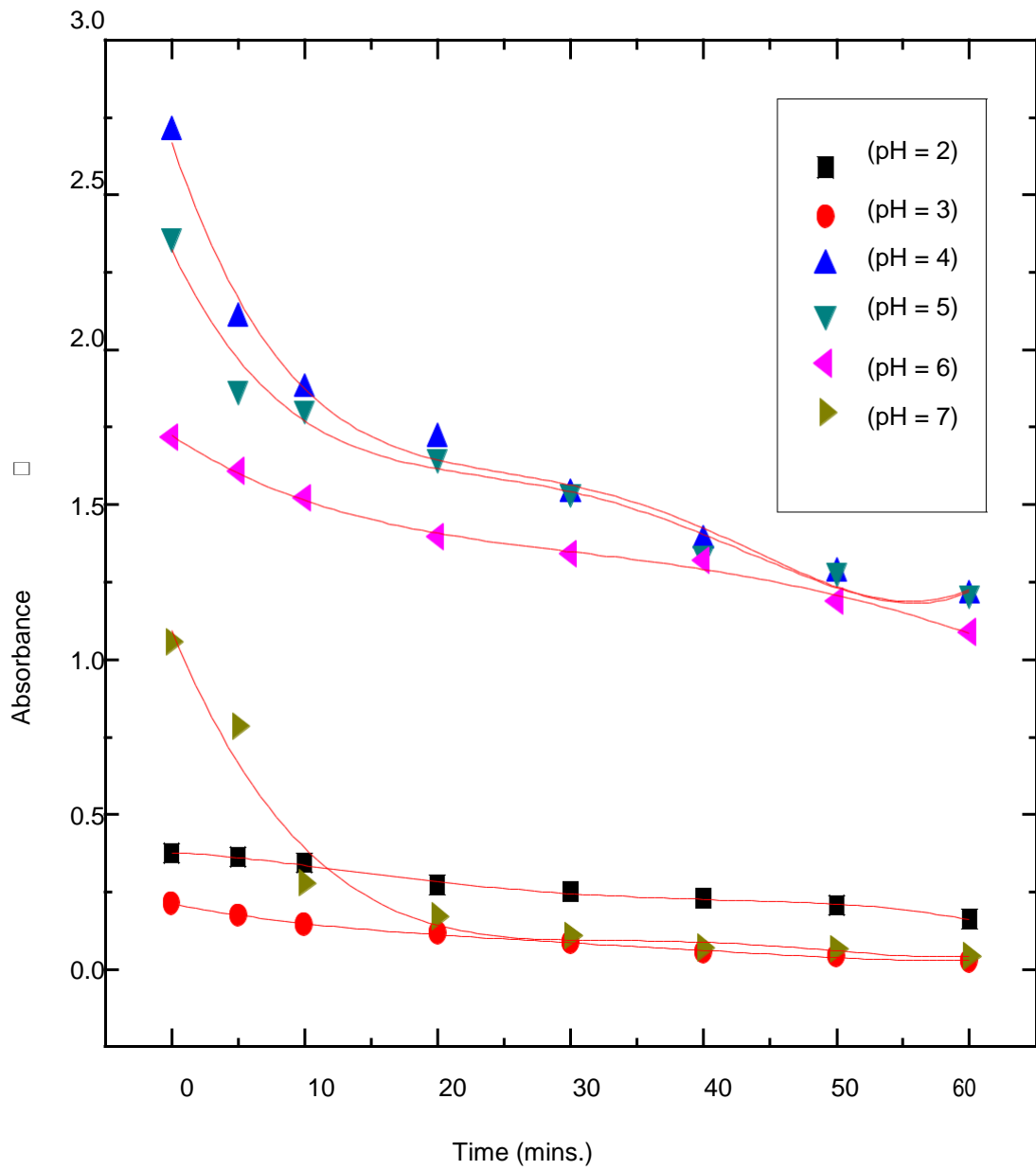
Fig 3.4(a) Change of absorption of the degraded solution with time using different pH of the solution.
