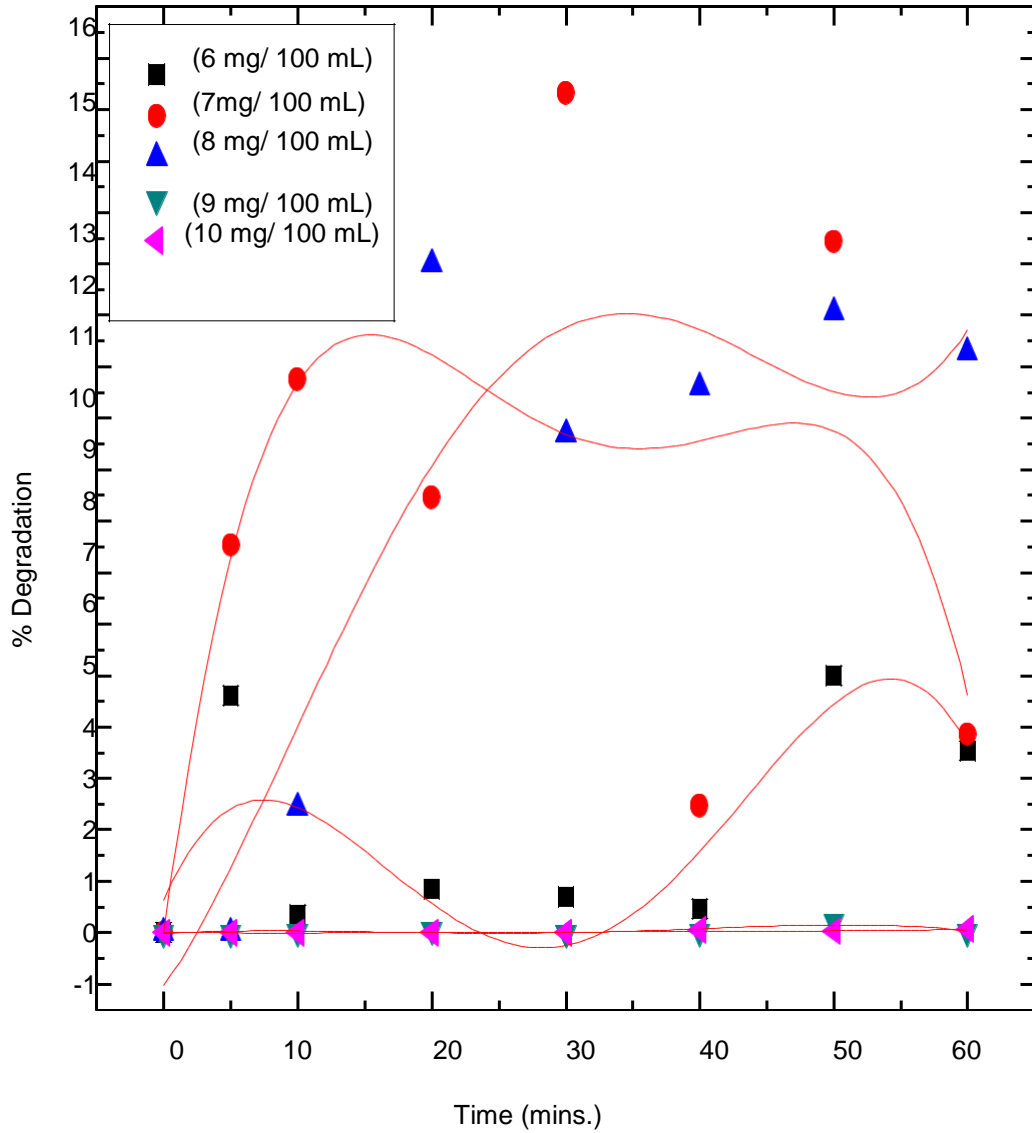
Fig: 3.2.1 (b) % of degradation of MO solution with time using different initial concentration
