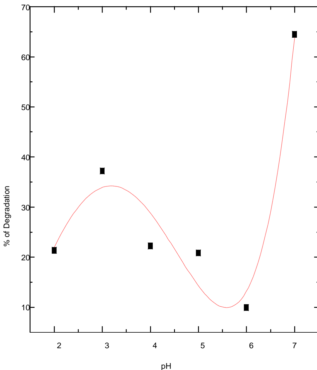
Fig 3.4.1(a) Effect of pH on percent degradation of MO during 60 minutes of irradiation
