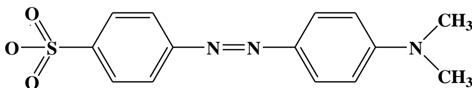
Scheme-01: Molecular Structure of Methyl Orange
