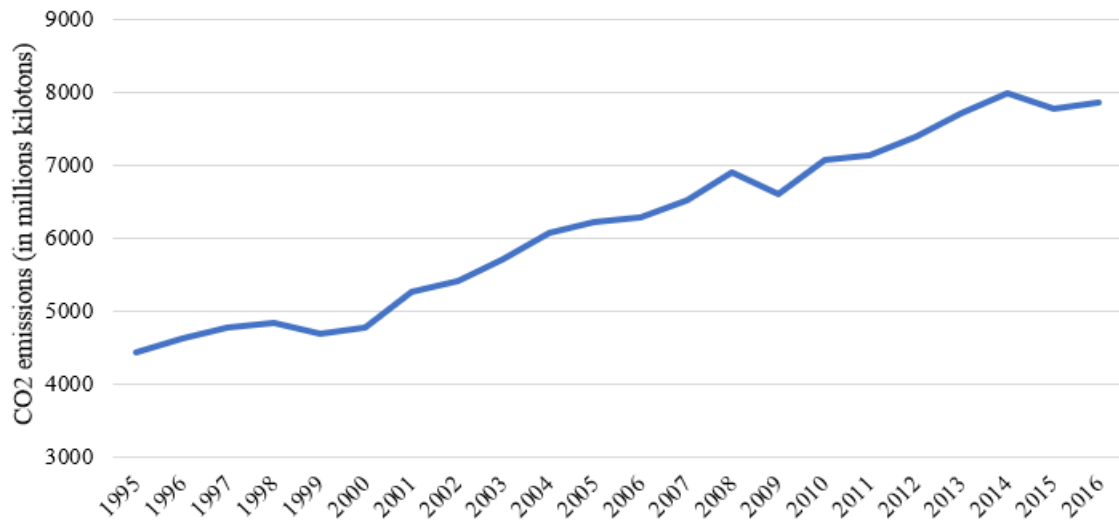
Figure 1 : Dynamic of CO 2 emissions over 1995-2016 in SSA.
